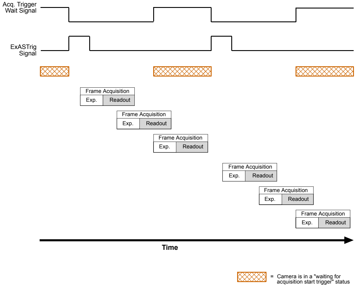
Fig. 50: Acquisition Trigger Wait Signal
