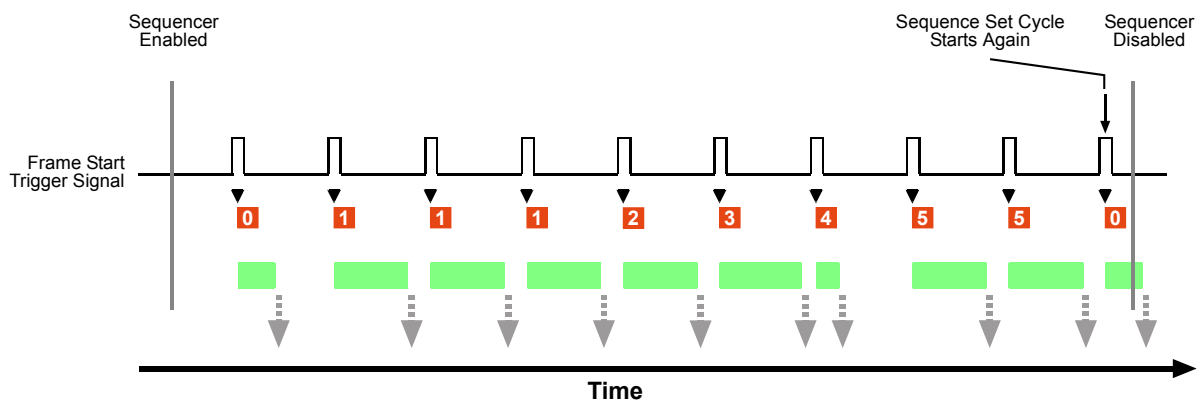
Fig. 58: Sequencer in Auto Sequence Advance Mode
