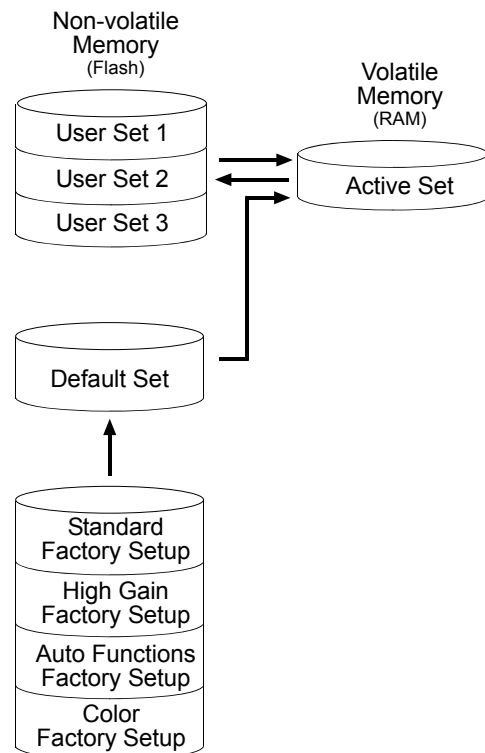
Fig. 79: Configuration Sets
