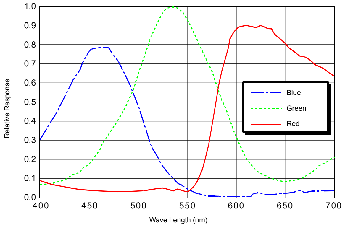
Fig. 10: piA2400-17gc Spectral Response
