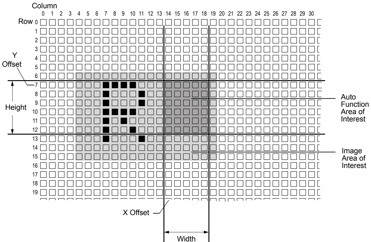
Fig. 71: Auto Function Area of Interest and Image Area of Interest
