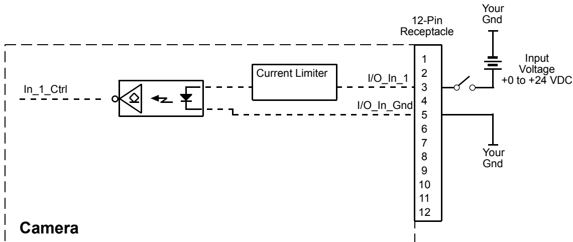
Fig. 25: Typical Voltage Input Circuit
