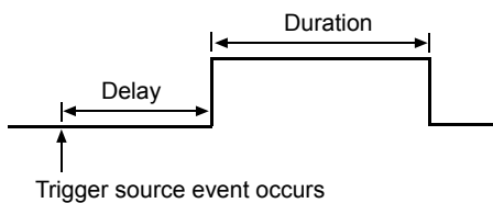
Fig. 30: Timer Signal
