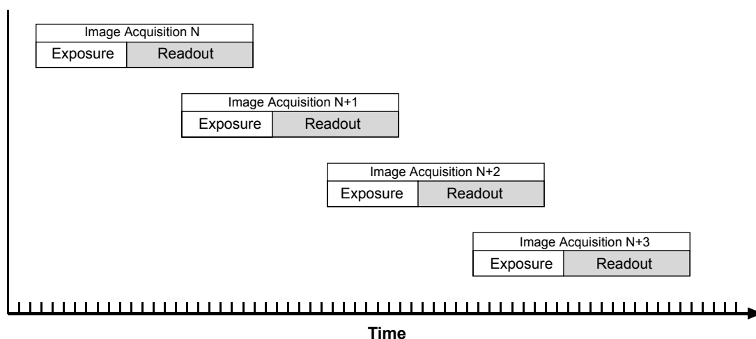
Fig. 47: Overlapped Exposure
