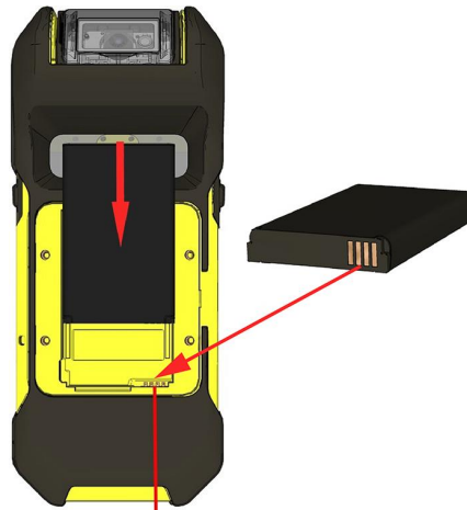
battery contacts
