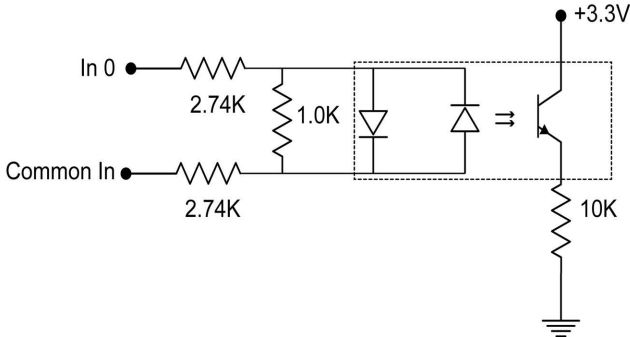
26.4V Max. across input pins - Transition approximately 12V (Min.)
