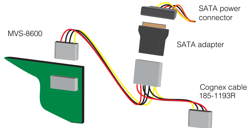
Figure 5. SATA adapter and power adapter cable
