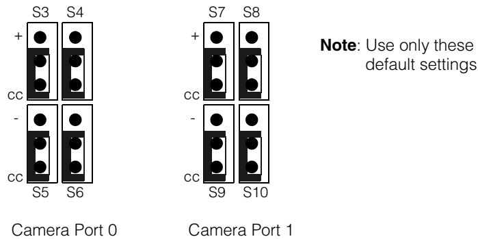
Figure 19. Jumpers S3-S10 factory default settings
