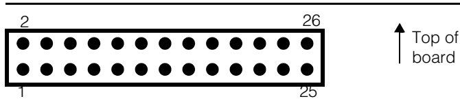
Figure 22. Pin numbering of the P4 and P6 connectors
