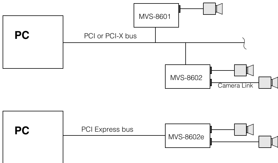
Figure 14. MVS-8600 overview
