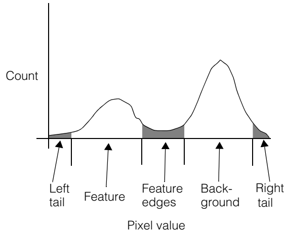
Figure 86. Pixel values in an image spread out the peaks of a histogram
