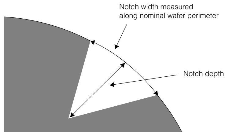
Figure 407. Notch width and depth
