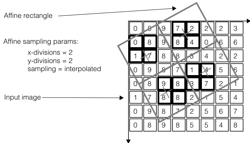
Figure 123. Large affine pixels
