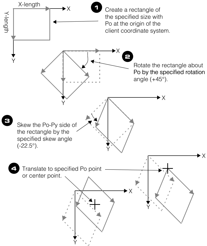
Figure 124. Creating an affine rectangle.
