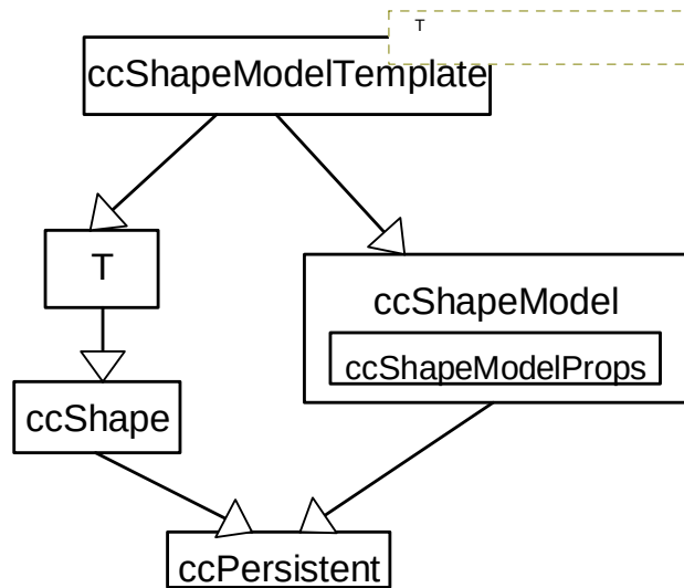
Figure 7. ccShapeModelTemplate<T> class inheritance hierarchy
