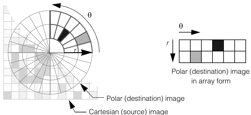
Figure 135. Cartesian source image mapped to polar destination image.
