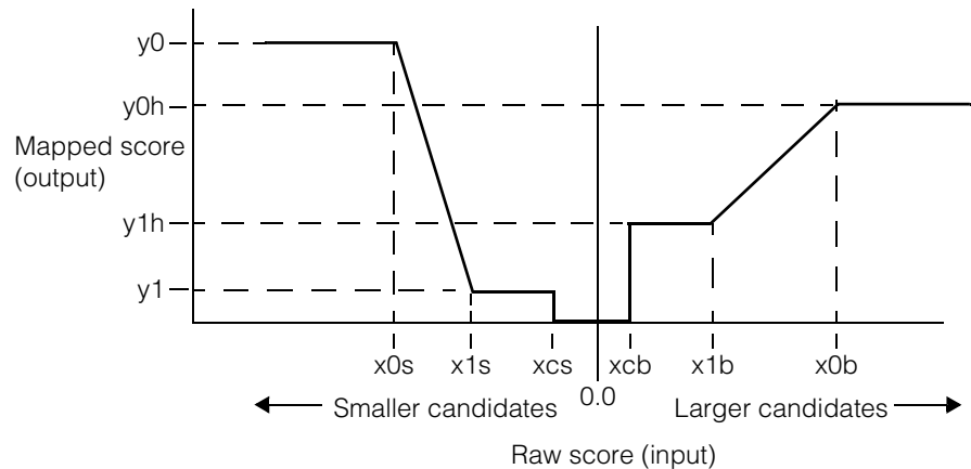
Figure 226. Two-sided scoring function with low output values in the center
