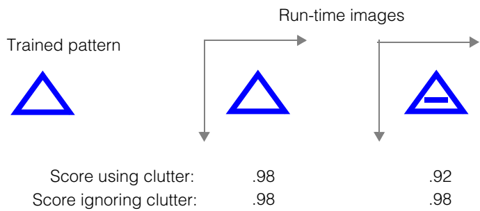
Figure 330. Computing score with and without clutter
