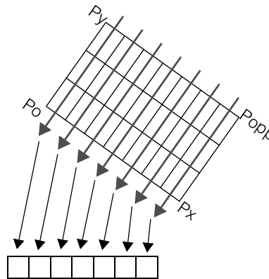
Figure 209. Project region defined by affine rectangle and sampling parameters
