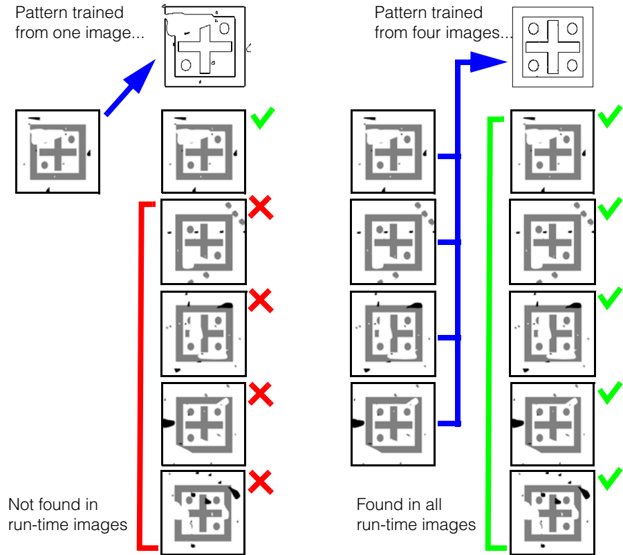
Figure 339. Composite model training from multiple degraded images
