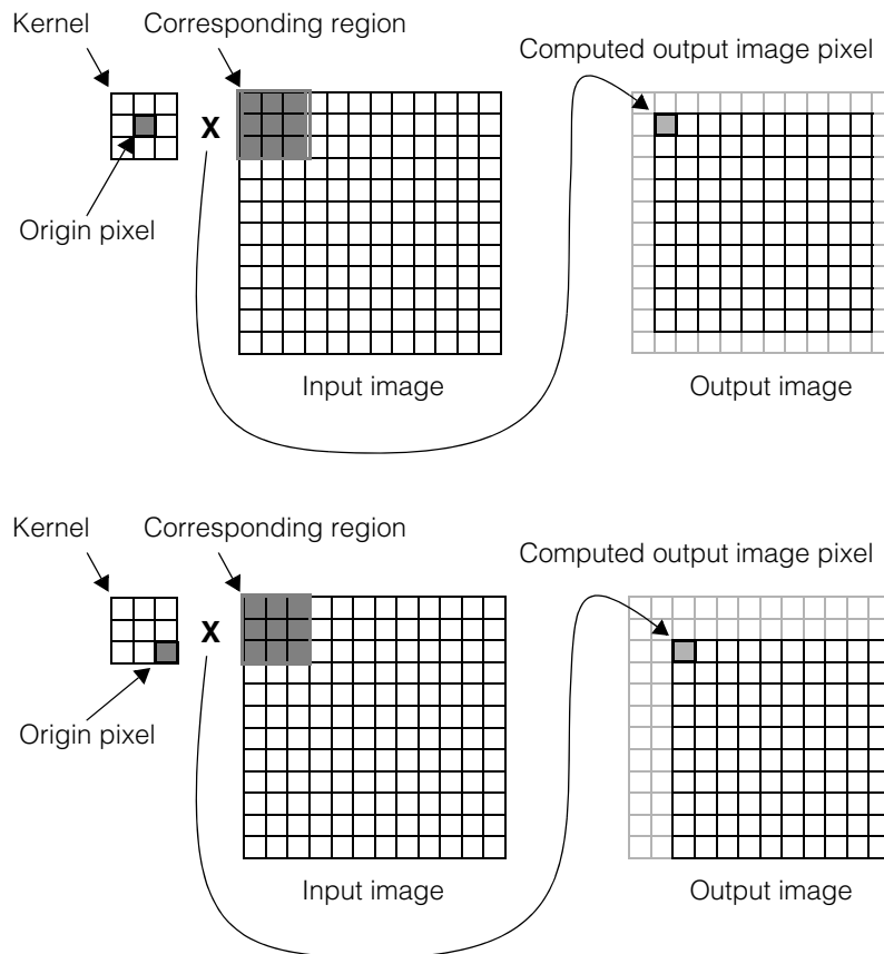
Figure 103. Kernel origin affects offset but not size of output image
