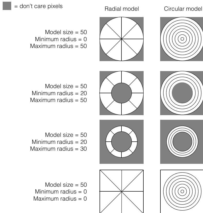
Figure 80. Minimum and maximum radius
