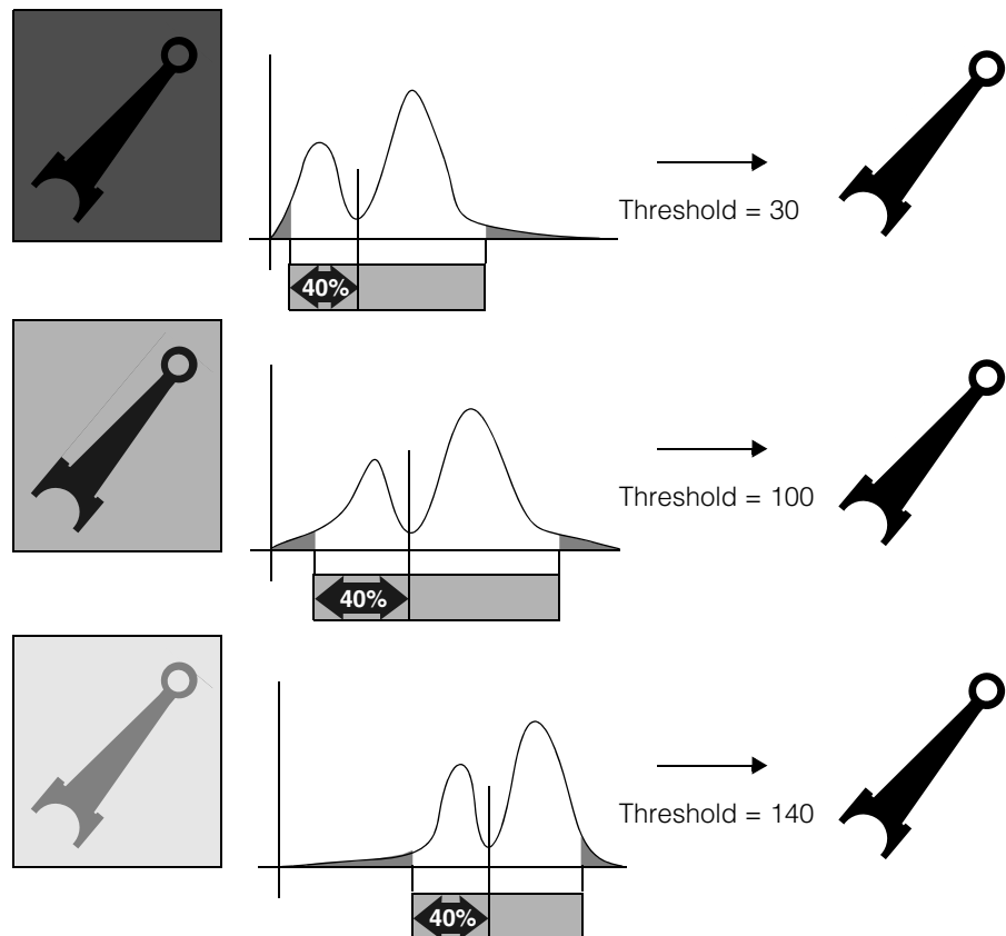
Figure 248. Relative threshold
