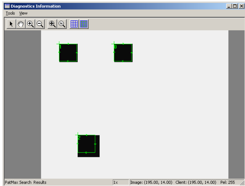
Figure 360. PatMax results
