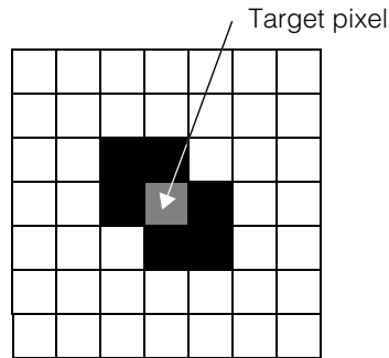
Figure 263. 6-way connectivity
