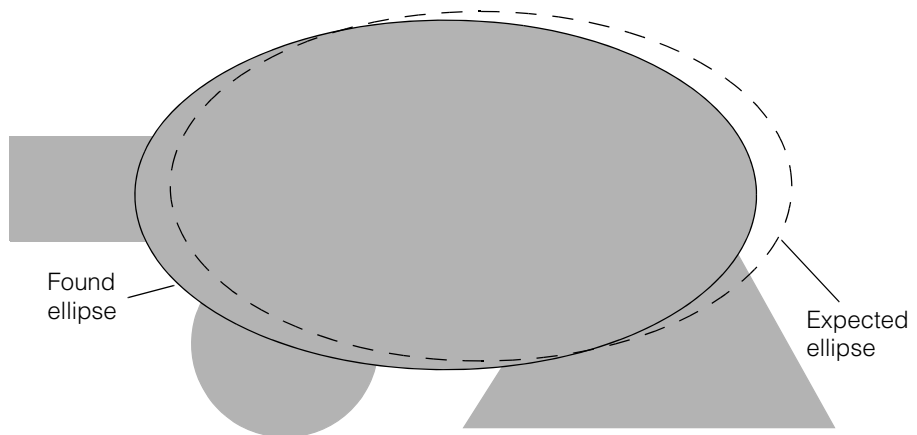
Figure 396. Found ellipse
