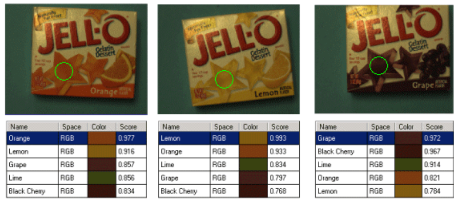
Figure 168. Classified images
