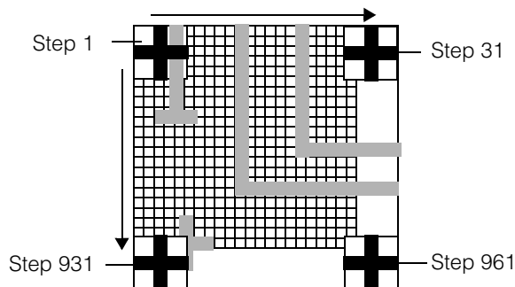
Figure 283. Exhaustive search
