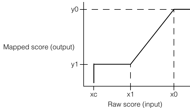
Figure 222. Scoring function
