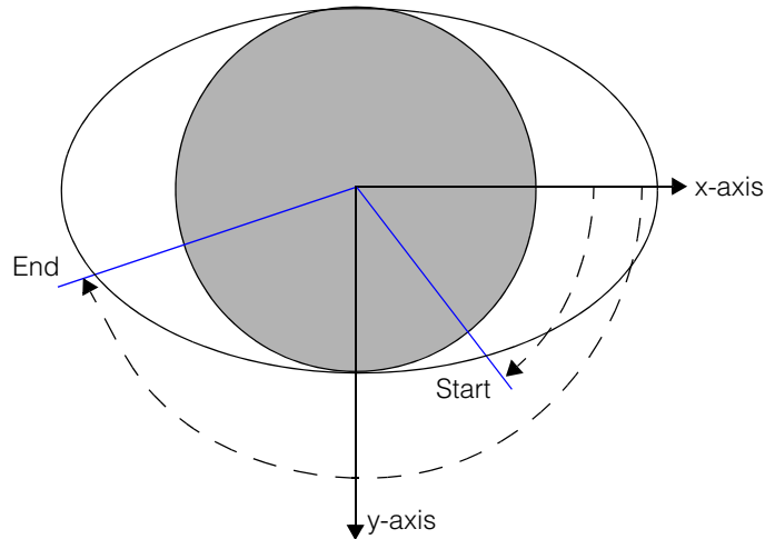
Figure 393. Ellipse angle range and the unit circle
