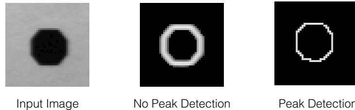
Figure 235. Peak detection
