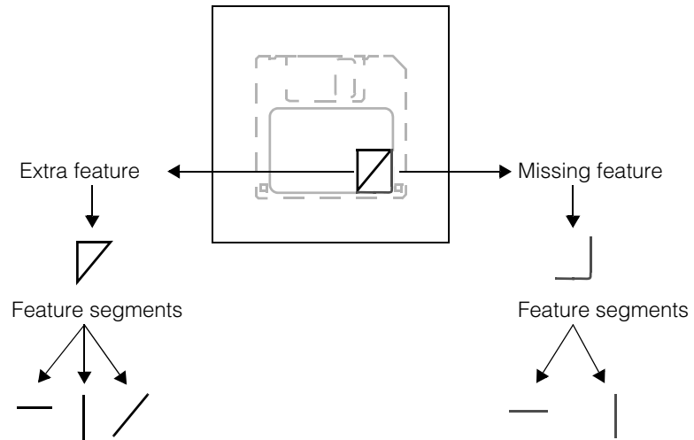
Figure 433. Segmenting features
