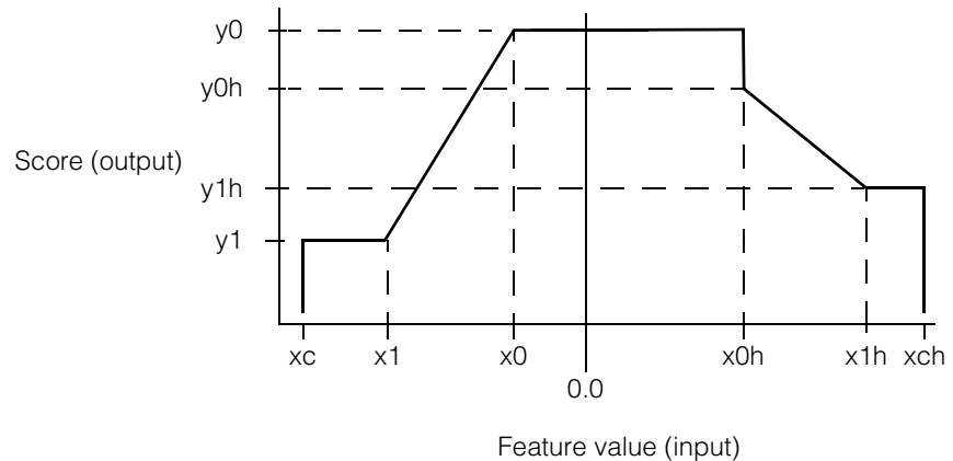
Figure 35. Two-sided scoring function
