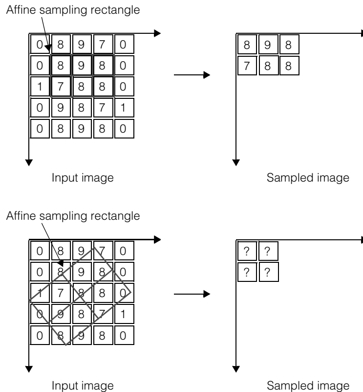
Figure 110. Orthogonal and non-orthogonal affine sampling rectangles
