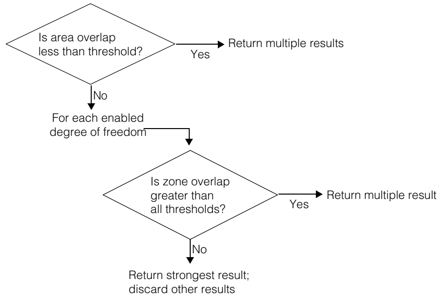
Figure 334. Overlap threshold processing
