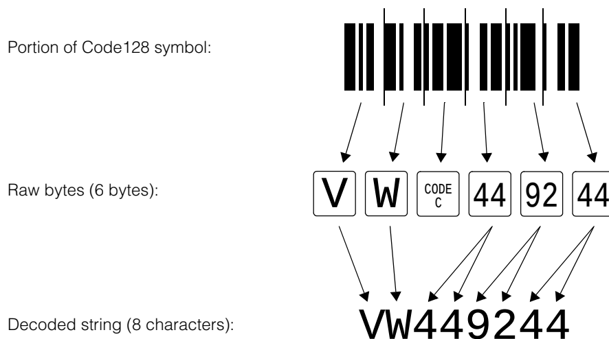
Figure 505. Decoding a Code128 symbol
