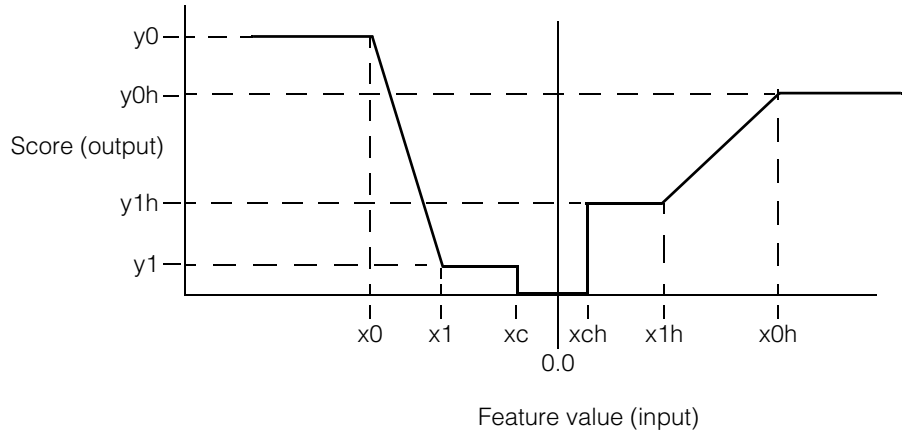
Figure 36. Two-sided scoring function with low output values in the center
