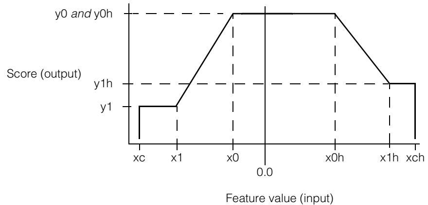
Figure 34. Two-sided scoring function
