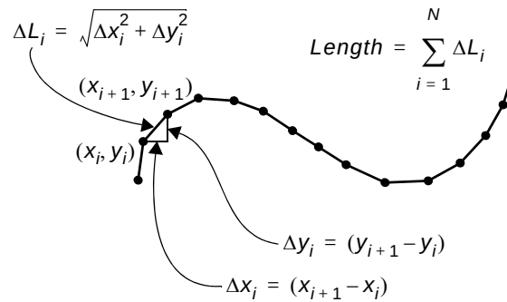
Figure 436. How the length of a feature boundary is computed
