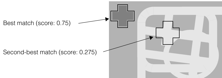
Figure 307. Estimating the confusion threshold
