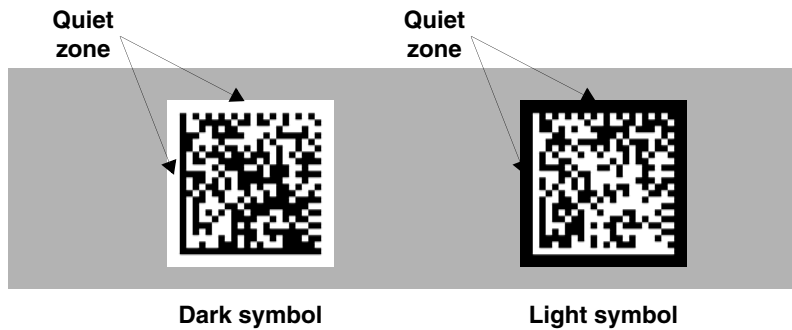
Figure 485. Dark vs. Light Data Matrix symbols
