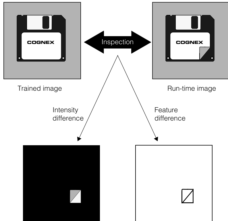
Figure 418. Intensity and feature difference
