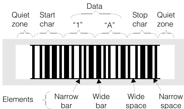
Figure 501. Bc39 barcode symbol structure
