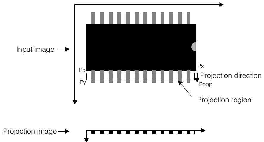
Figure 130. Unrotated projection region
