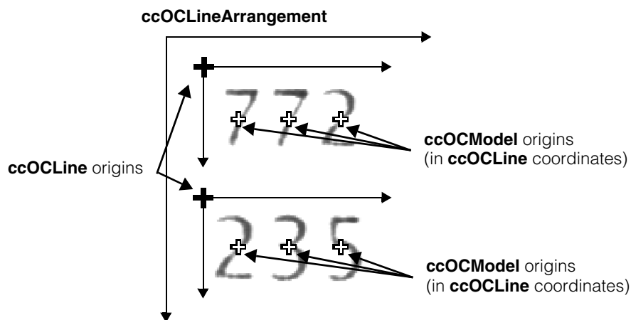
Figure 521. An arrangement of characters and lines
