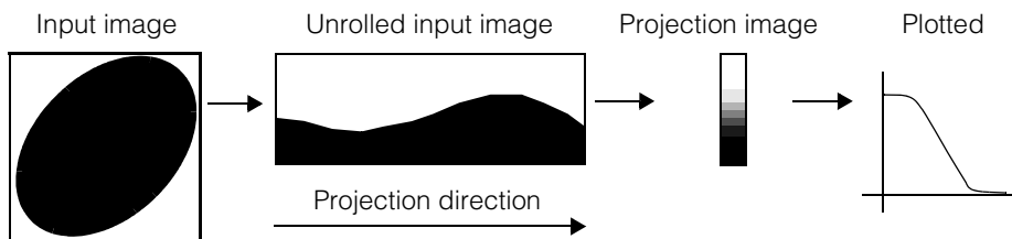
Figure 75. Circular projection region applied to eccentric object
