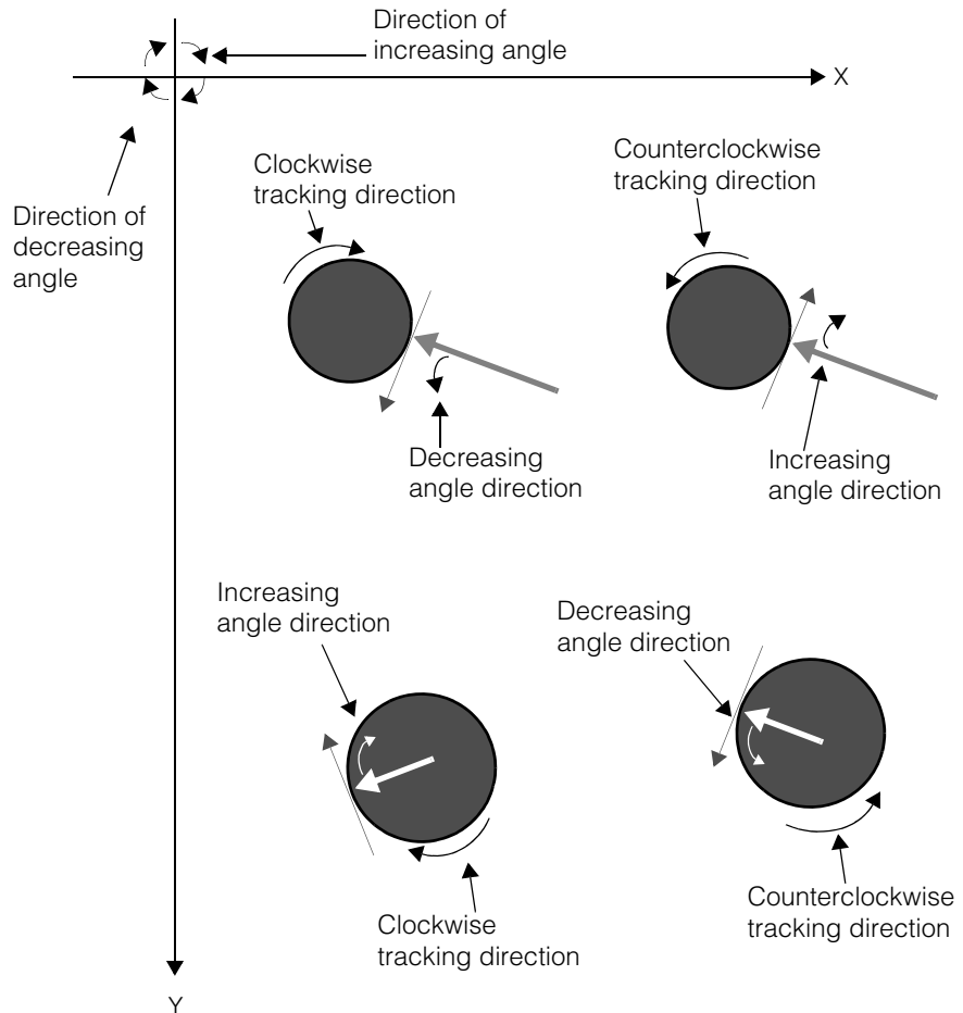
Figure 278. Tracking directions in left-handed coordinate system
