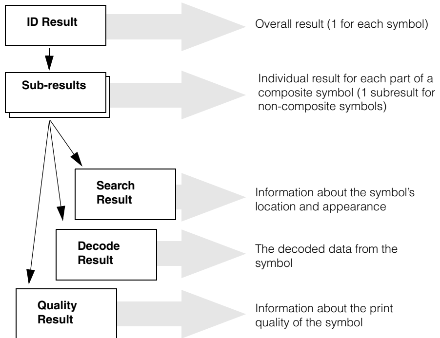
Figure 465. ID Tool results
