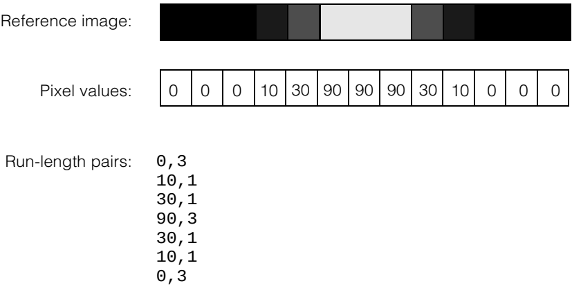
Figure 218. Run-length encoded reference image
