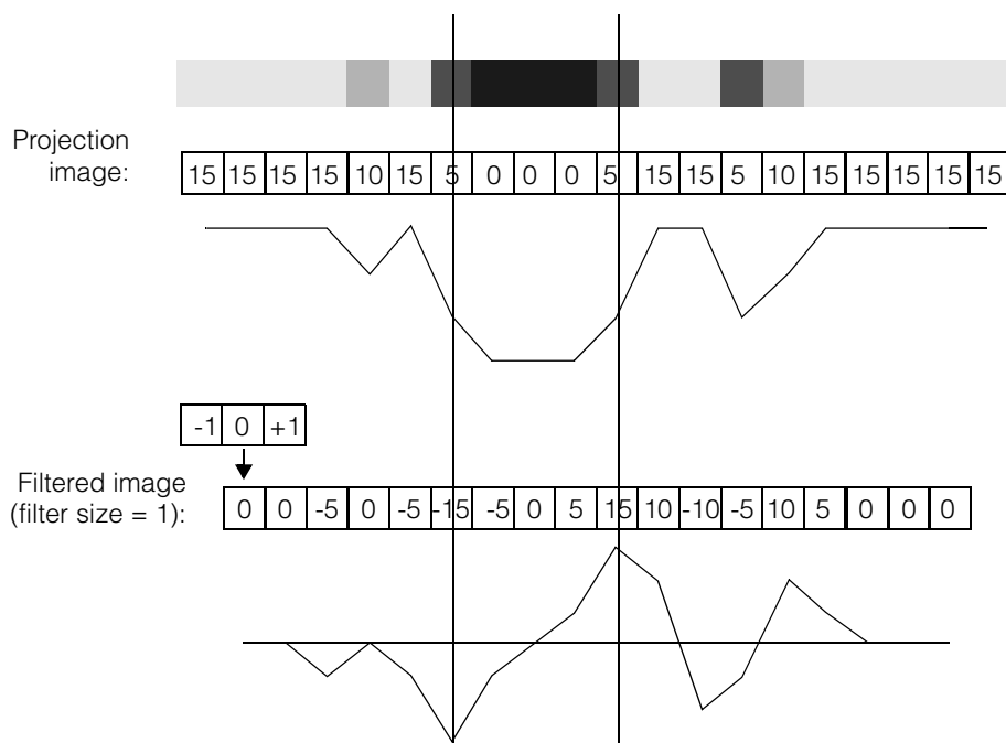
Figure 204. Filtering with filter size of 1
