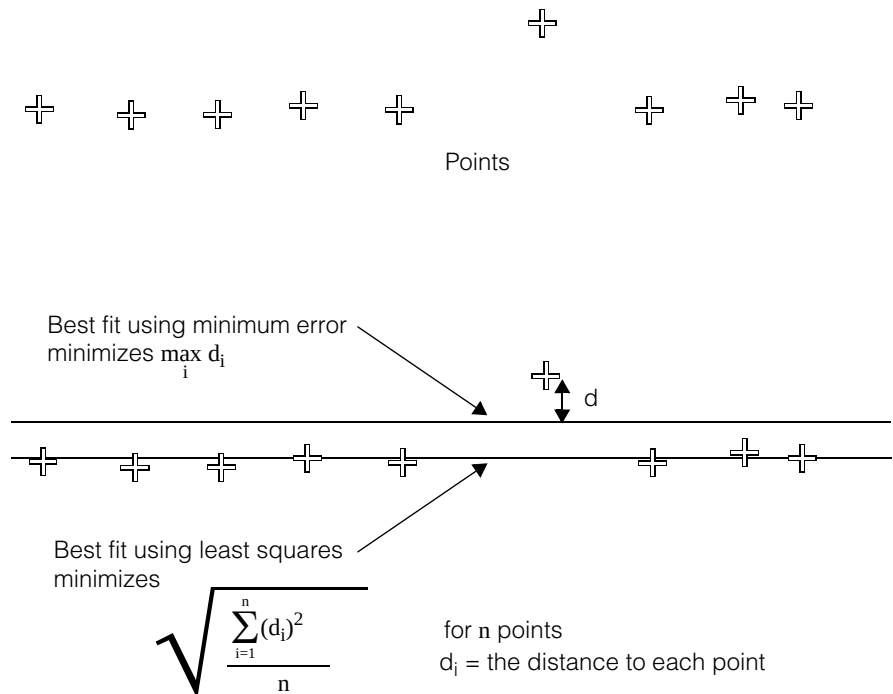
Figure 15. Fitting a line to points using least squares and minimum error methods
