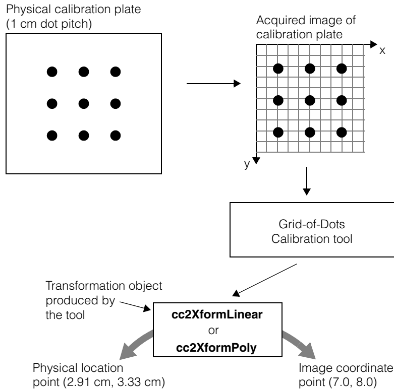
Figure 171. Grid-of-dots calibration
