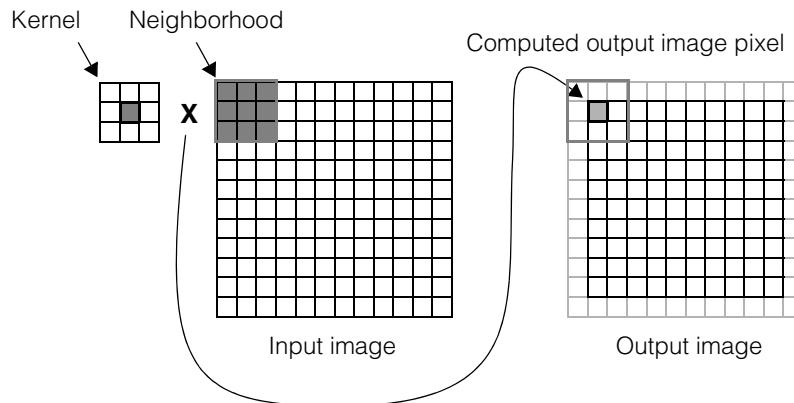
Figure 45. Kernel, neighborhood, and output image
