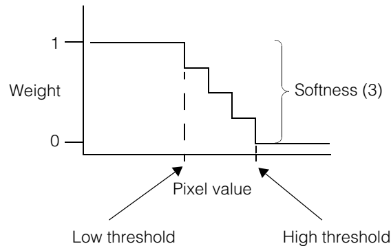
Figure 259. Soft binary threshold with invert flag set
