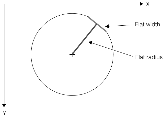
Figure 408. Specifying wafer flat dimensions
