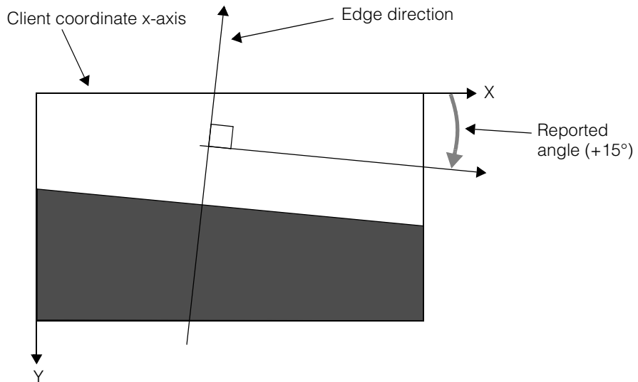
Figure 151. Reported scene angle is edge angle + 90^\circ
