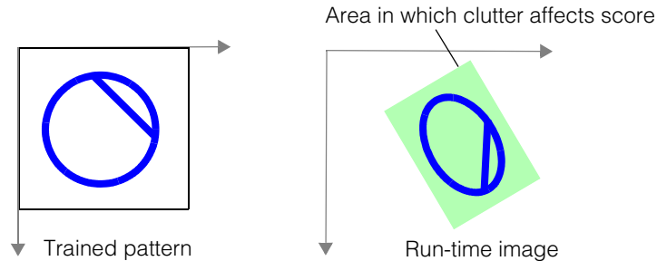
Figure 324. Area considered when computing clutter
