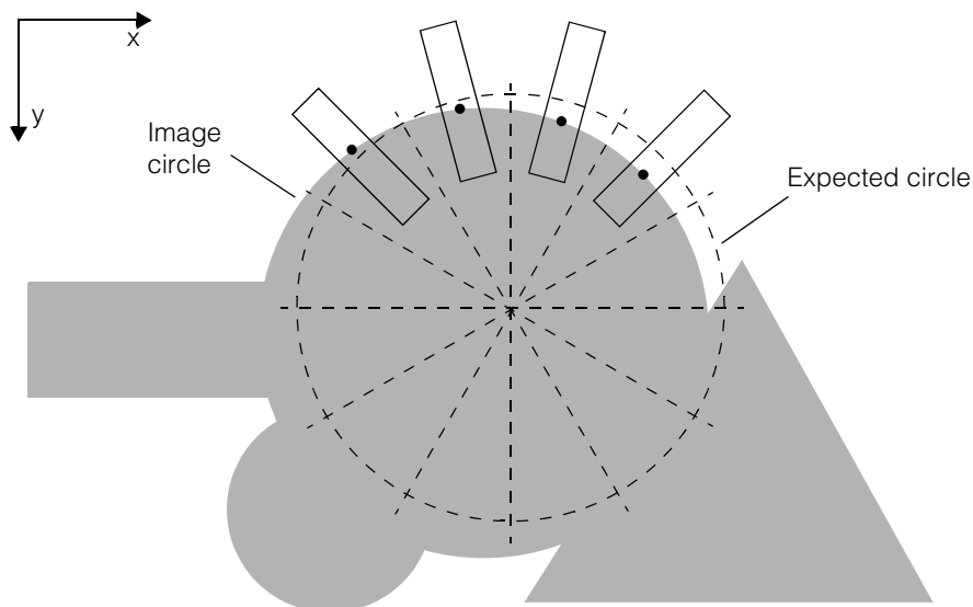
Figure 389. Example, found edges
