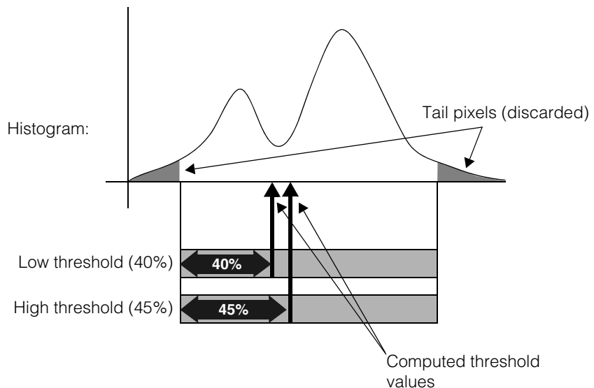
Figure 249. Computing relative soft threshold values of 40% and 45%
