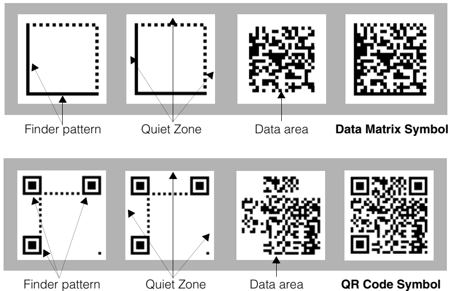
Figure 483. Data Matrix and QR Code symbols
