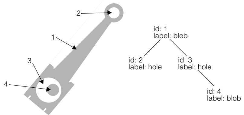
Figure 257. Blob topology described using a tree structure
