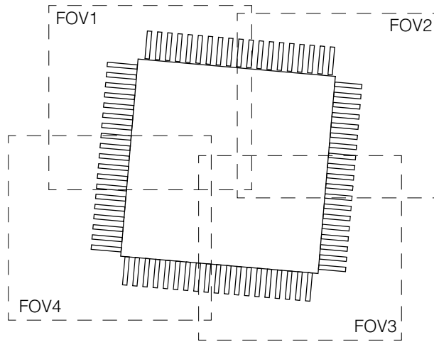
Figure 42. Example scene captured with four images
