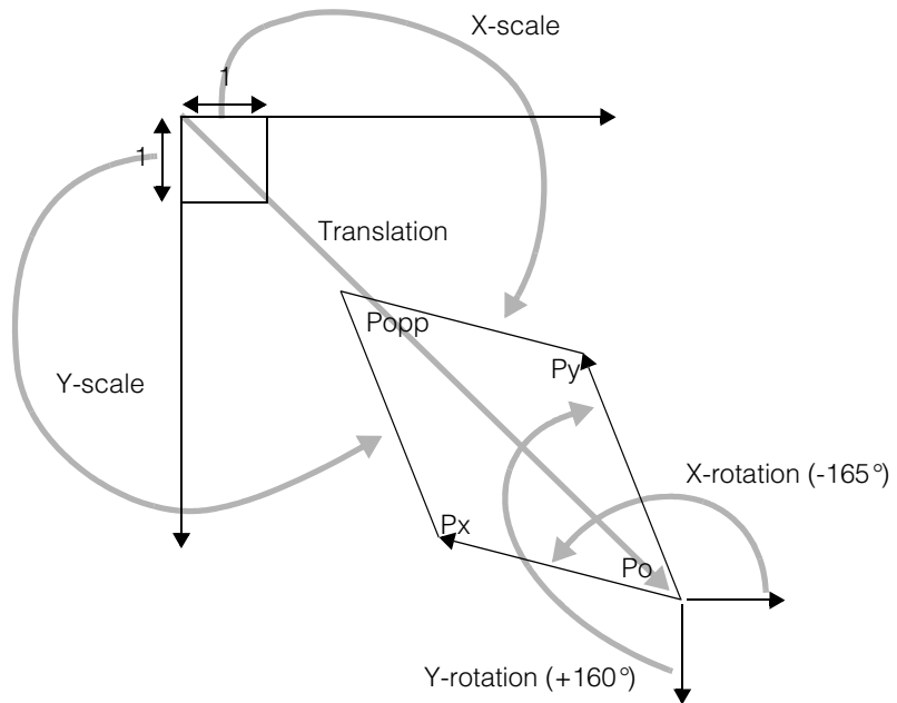
Figure 116. Changing vertices' locations by changing x rotation, y rotation, and translation
