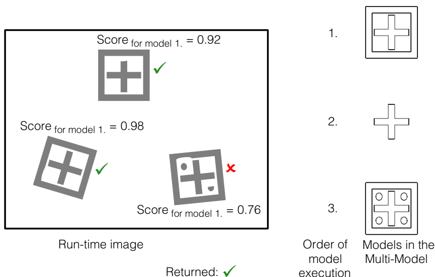
Figure 348. Multi-Model pattern matching using a confusion threshold
