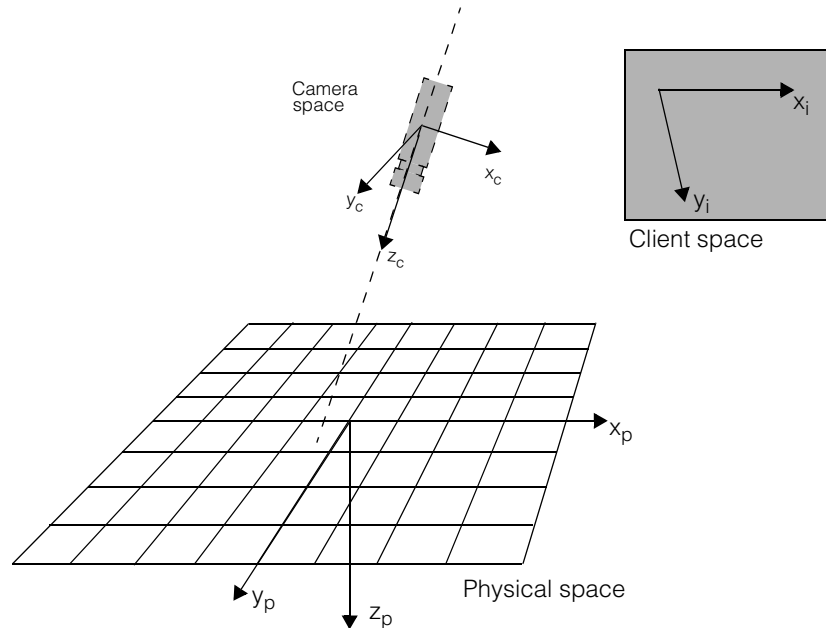
Figure 172. Calibration coordinate systems
