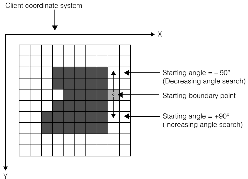
Figure 275. Starting point in track-only mode
