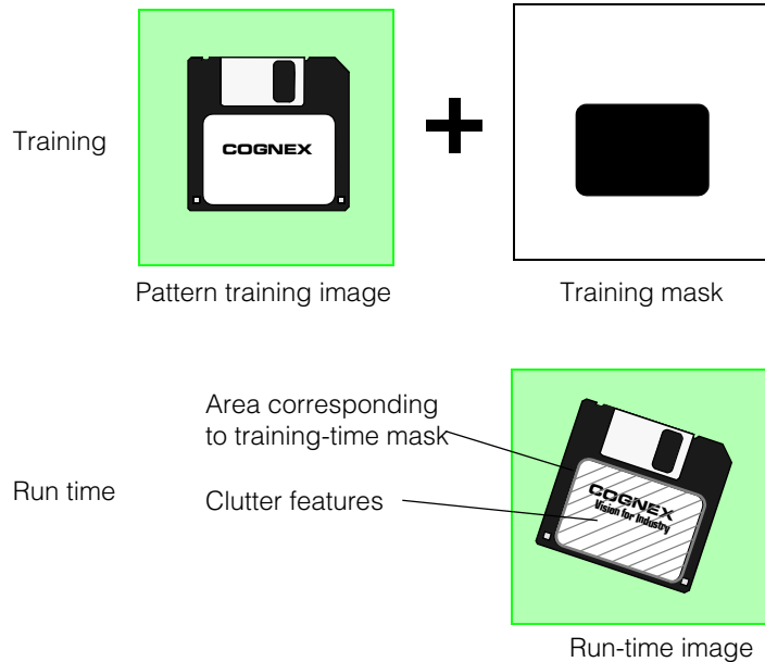
Figure 332. Clutter features and masking
