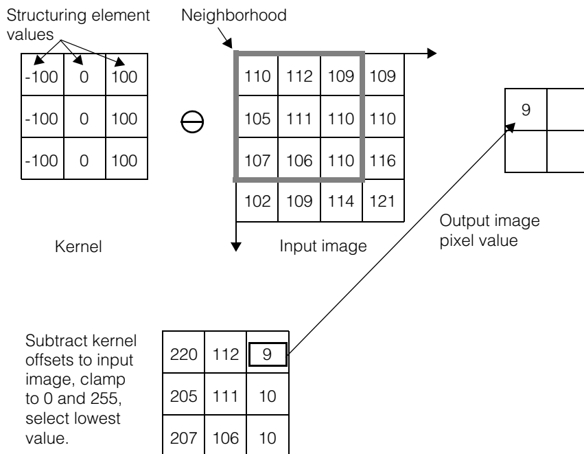
Figure 49. Example of a 3x3 erosion for a single destination pixel
