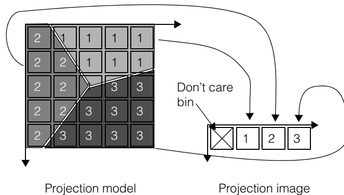
Figure 68. Projection Model
