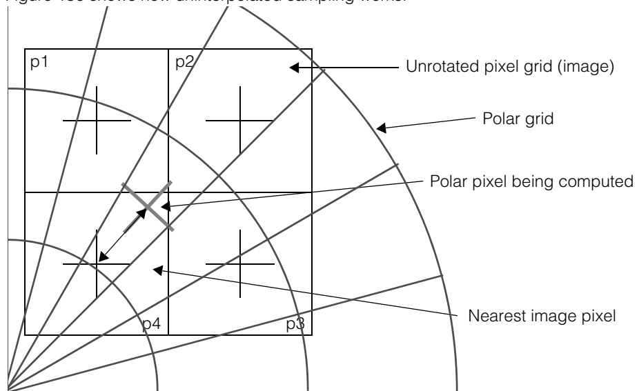
Figure 136. Uninterpolated sampling
