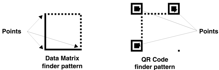
Figure 484. Point locations in Data Matrix and QR Code symbols
