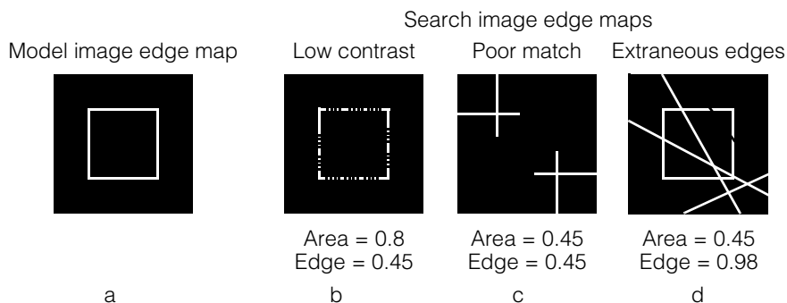
Figure 298. Area score and edge score for nonlinear search
