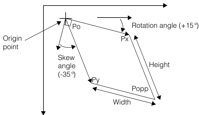
Figure 119. Affine rectangle specified by origin, size, and angles of skew and rotation
