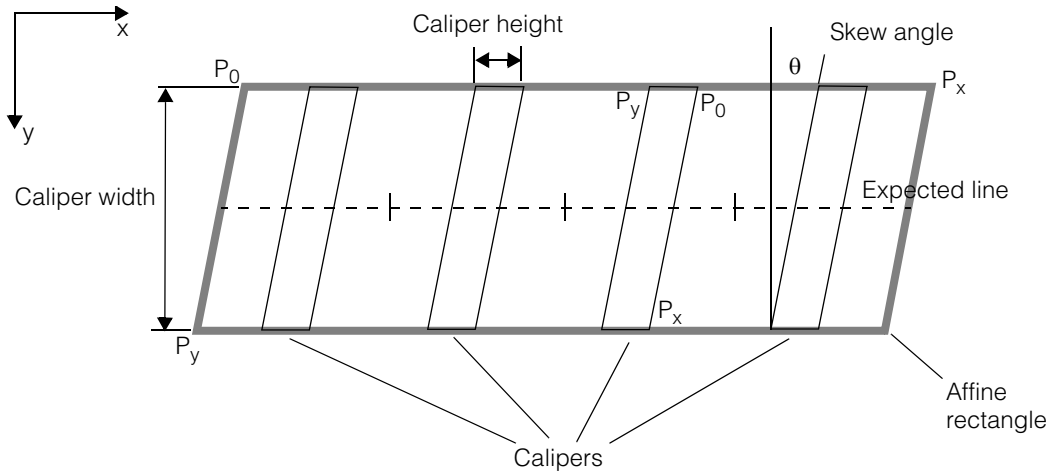
Figure 382. Skewed calipers
