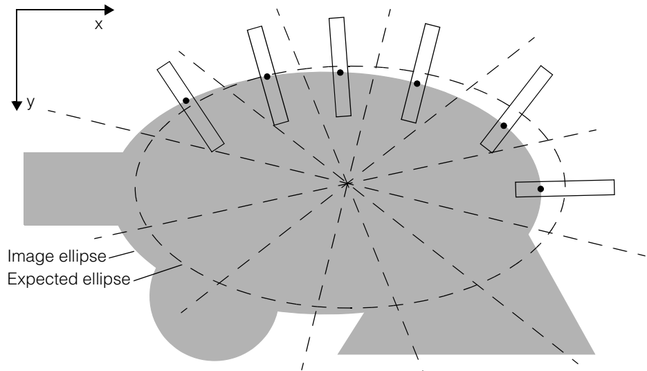
Figure 395. Example, found edges
