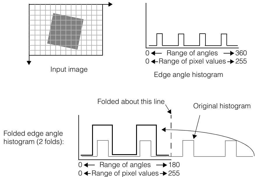
Figure 154. Folding the edge angle histogram
