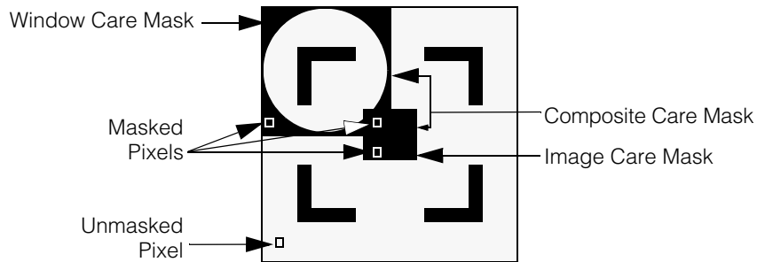
Figure 403. Example of composite care mask
