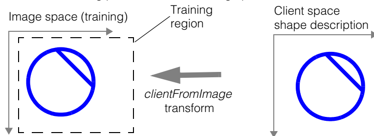
Figure 349. clientFromImage transform, shape training
