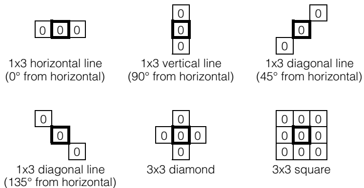
Figure 60. Pre-defined structuring element library
