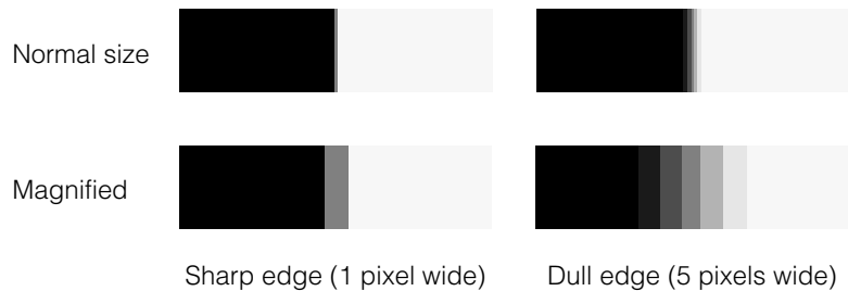
Figure 214. Sharp and dull edges
