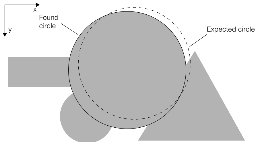
Figure 390. Example, found circle
