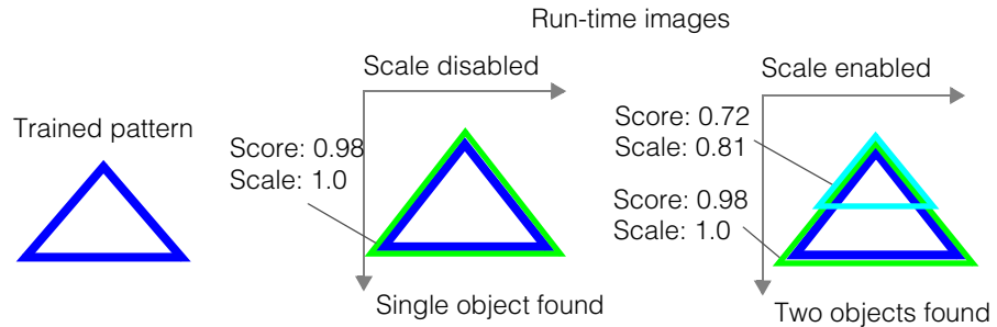
Figure 326. Image confusion increased with larger run-time space
