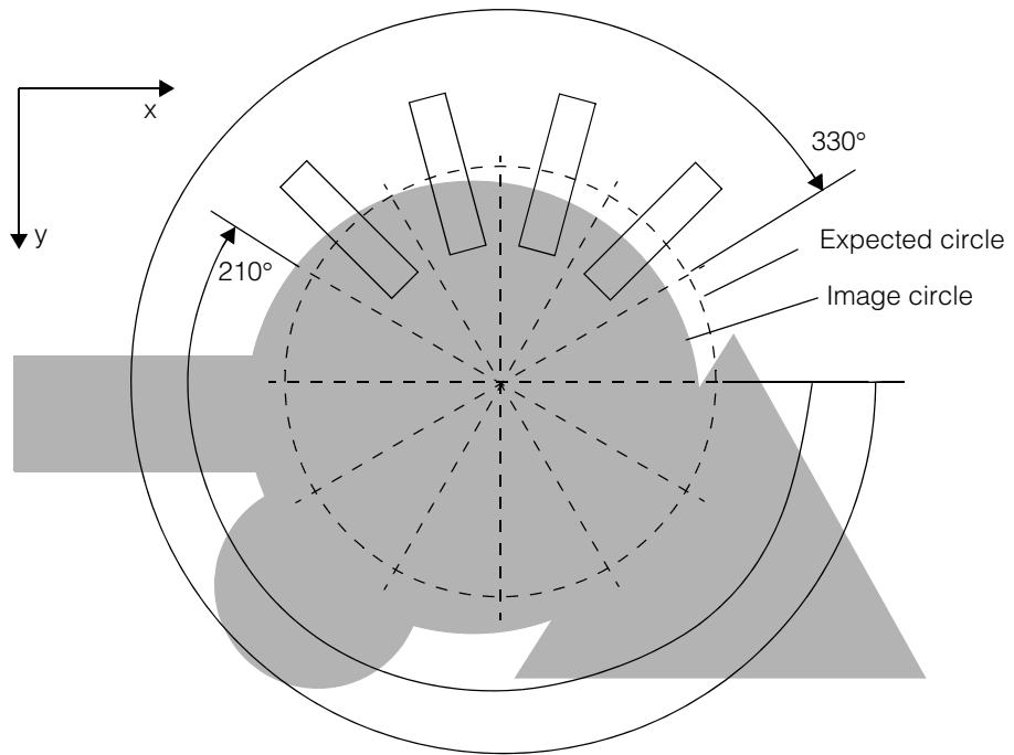
Figure 388. Example of expected circle and four calipers
