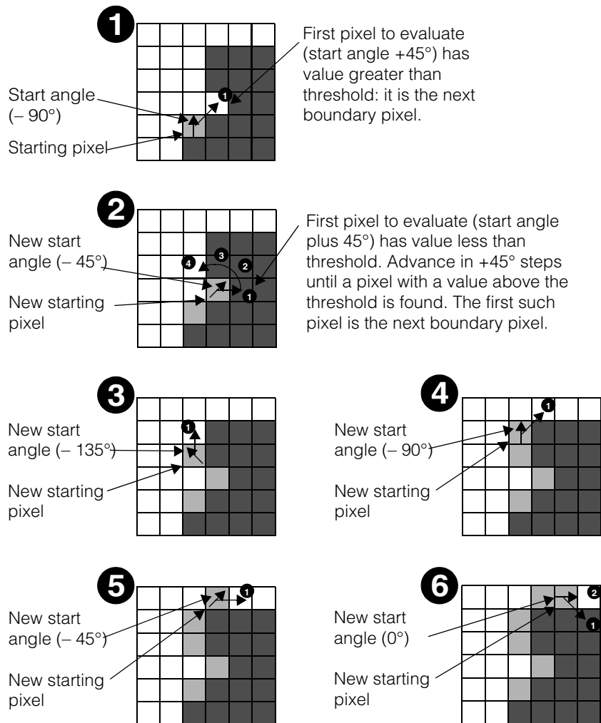
Figure 268. Tracking the object boundary
