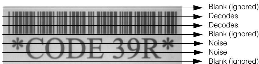
Figure 502. Scan lines crossing a barcode
