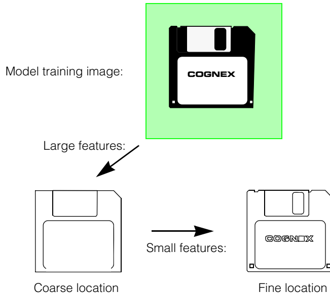
Figure 371. Large features used for coarse location and small features for fine location
