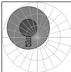
Figure 138. Object, at 0 degrees, rotated 75 degrees, and translated in x-y
