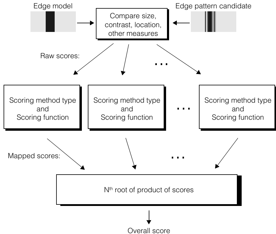
Figure 227. Scoring an edge pattern candidate
