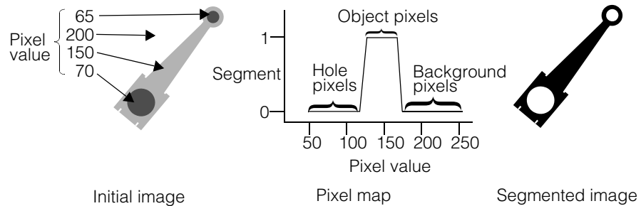
Figure 251. Segmenting an image with a pixel map
