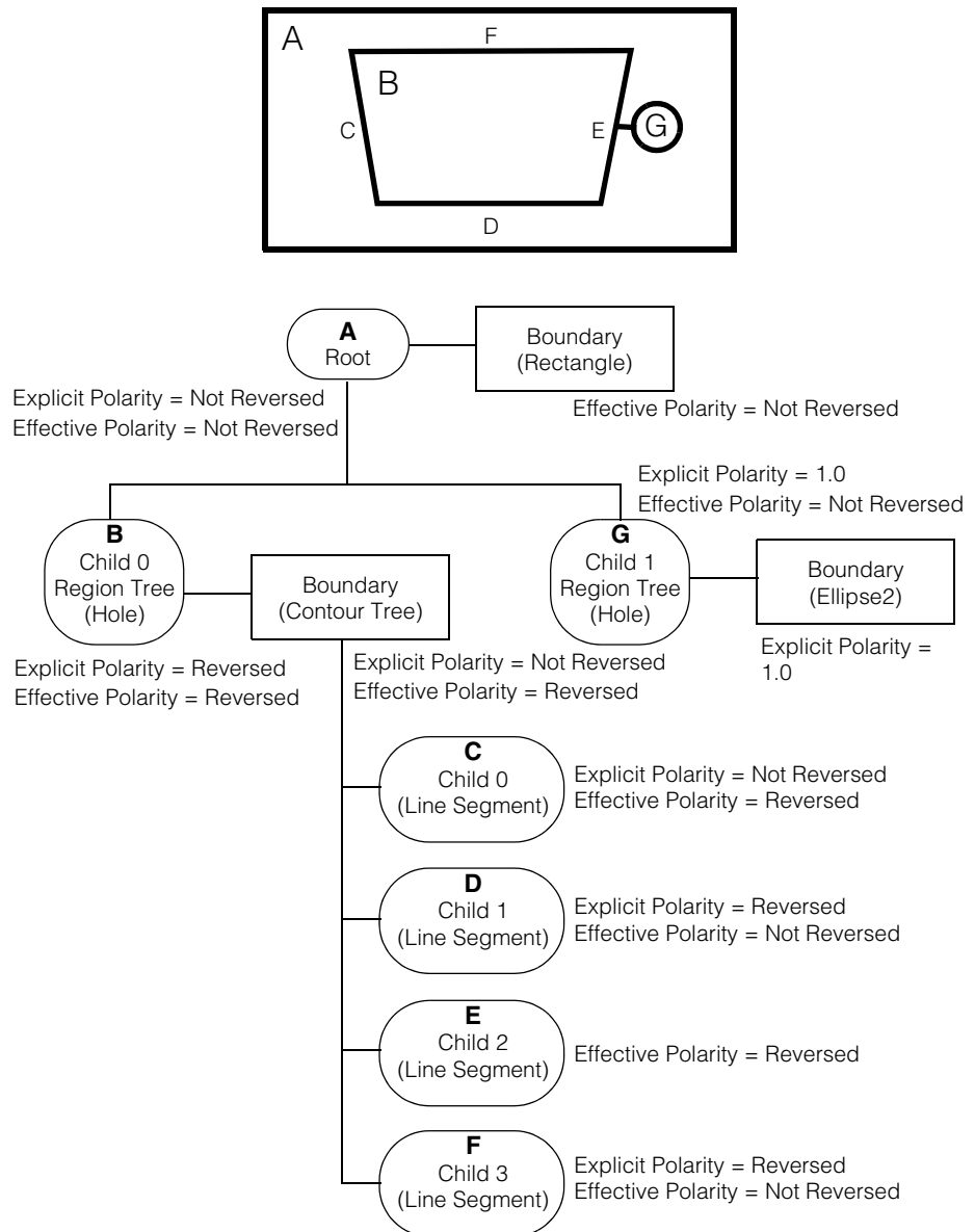
Figure 10. Effective polarities of individual nodes in a region tree shape description
