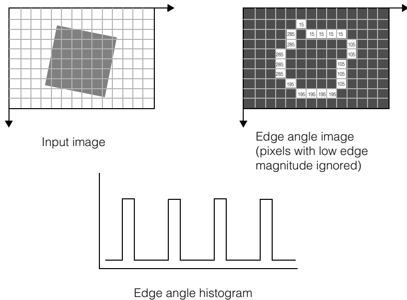
Figure 153. Reinforcing edges
