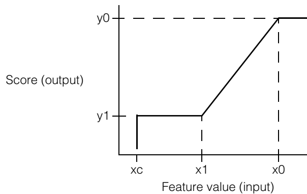
Figure 26. Scoring function
