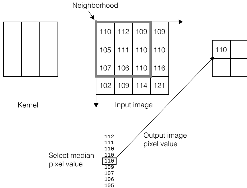
Figure 47. Median filtering
