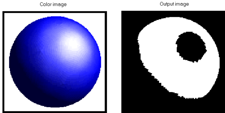
Figure 165. Hard threshold
