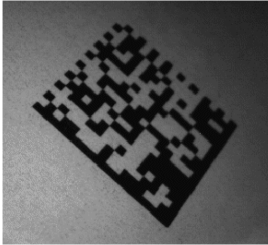
Figure 499. Perspective distortion
