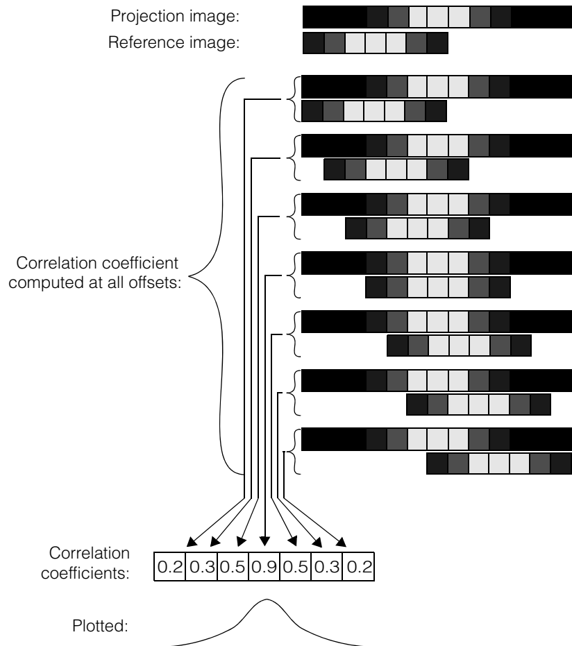
Figure 207. Correlation mode pattern location
