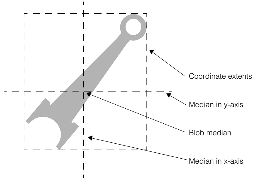
Figure 256. Blob nongeometric properties
