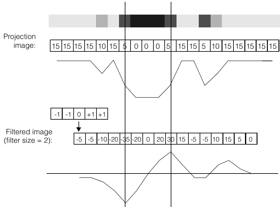
Figure 205. Filtering with filter size of 2
