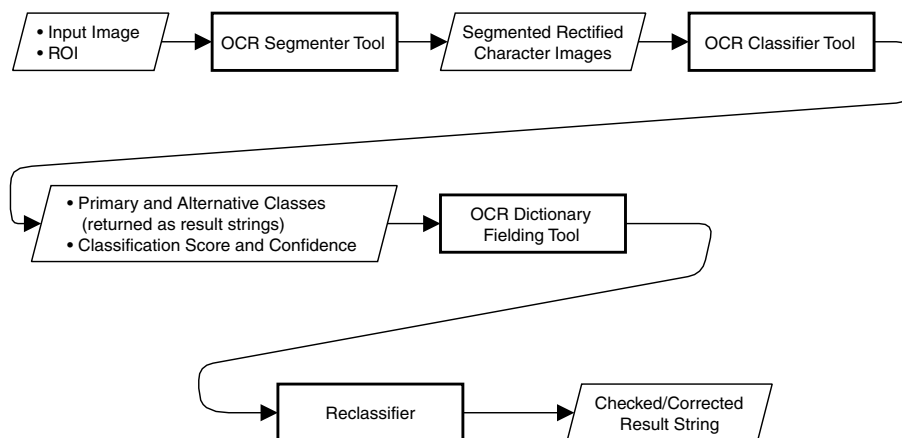
Figure 508. OCR process
