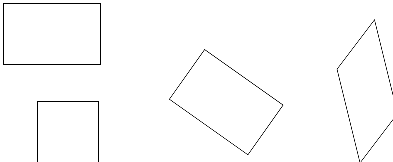
Figure 107. Affine rectangles
