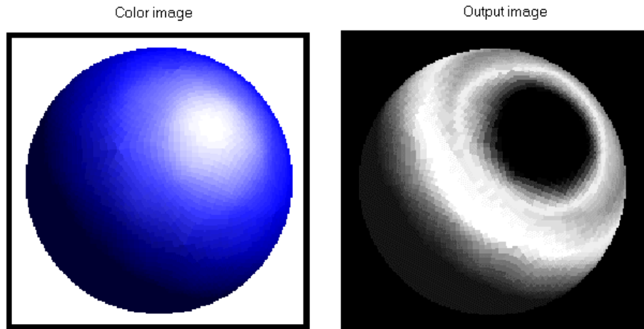
Figure 166. Soft threshold
