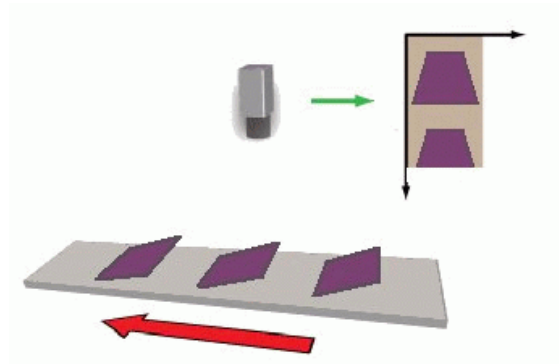
Figure 191. Perspective distortion
