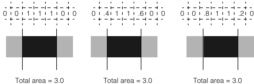
Figure 244. Pixel weighting
