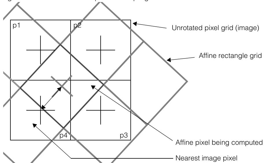
Figure 111. Uninterpolated sampling
