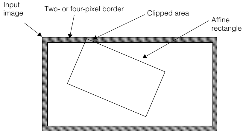
Figure 121. Clipping.
