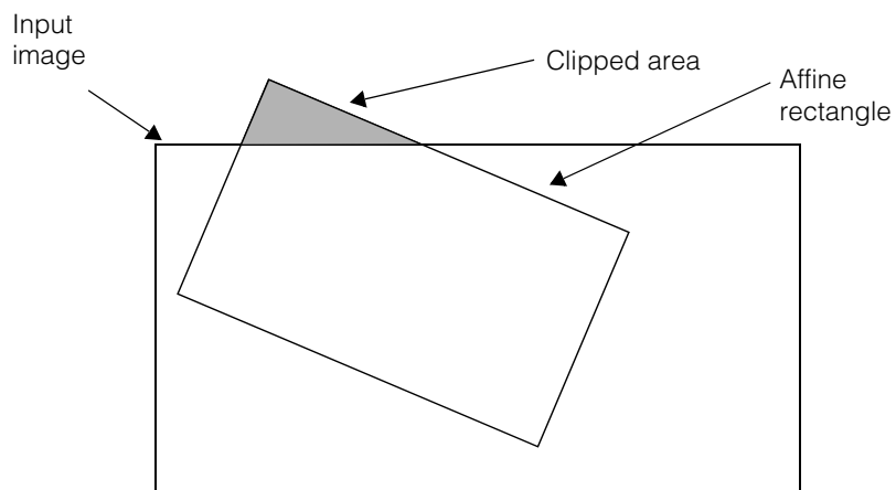
Figure 120. Clipping.
