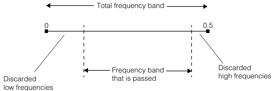
Figure 100. eBandPassFiltering mode
