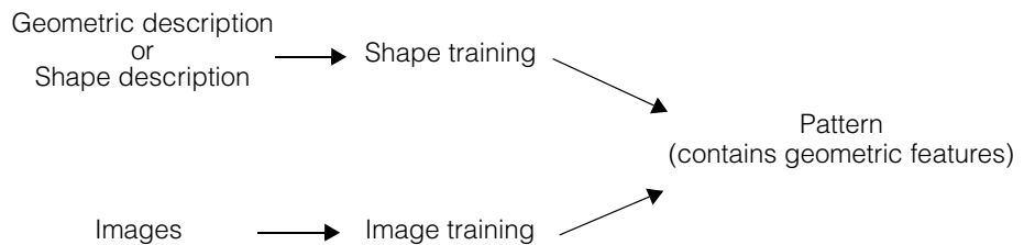
Figure 309. PatMax training
