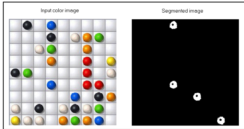
Figure 161. Color segmentation
