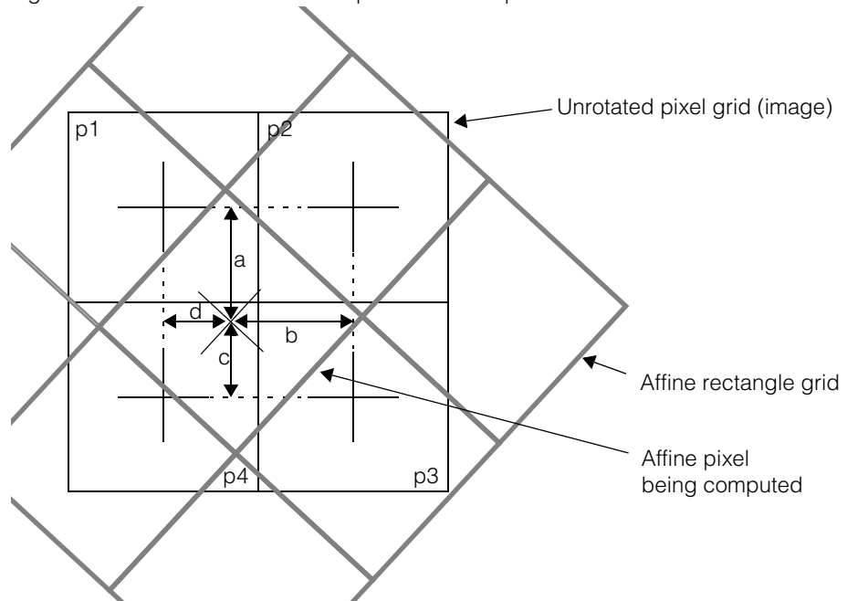
Figure 113. Bilinear interpolation
