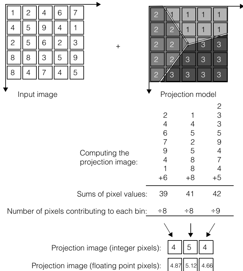
Figure 70. Normalized projection
