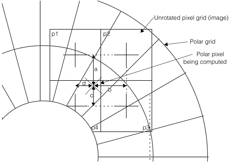
Figure 137. Bilinear interpolation
