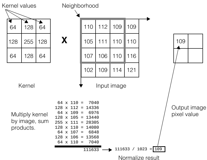
Figure 46. Discrete convolution
