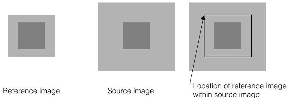
Figure 413. Image Registration
