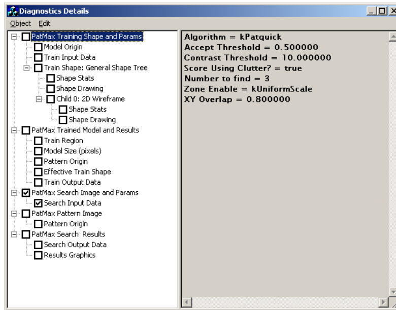
Figure 362. Complete diagnostics hierarchy
