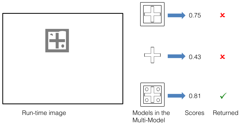
Figure 345. Multi-Model pattern matching with added Composite Models
