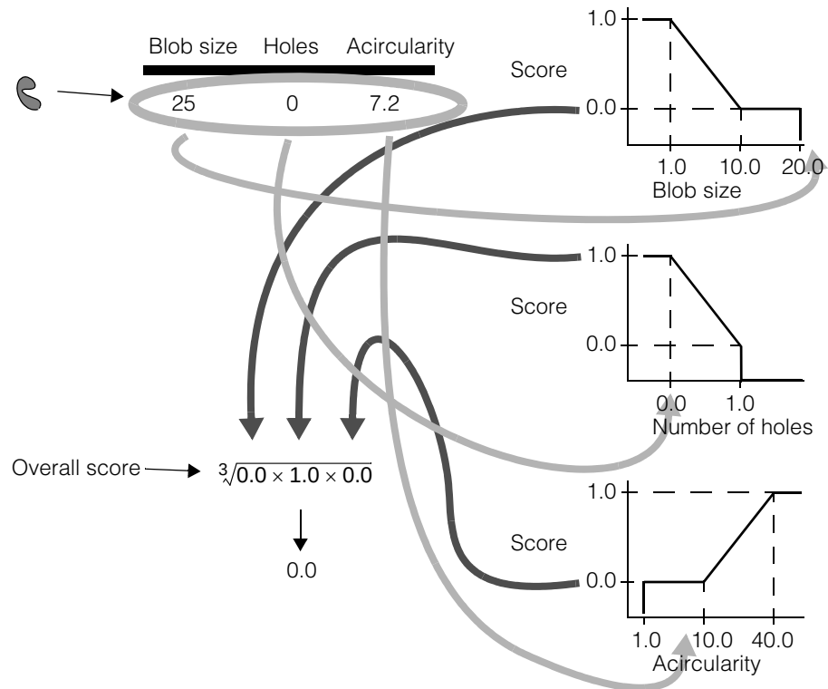
Figure 28. Applying the rule to a single feature vector
