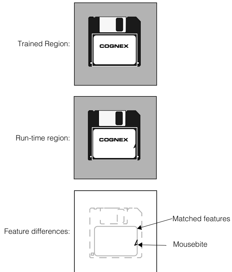
Figure 434. Mousebite
