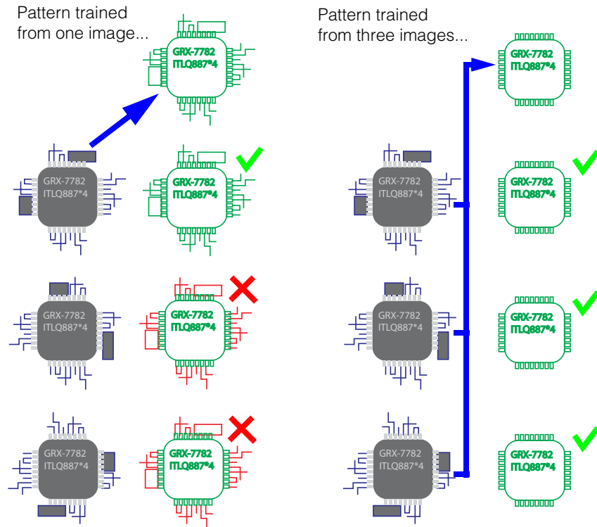
Figure 341. PatMax Composite for parts with different backgrounds
