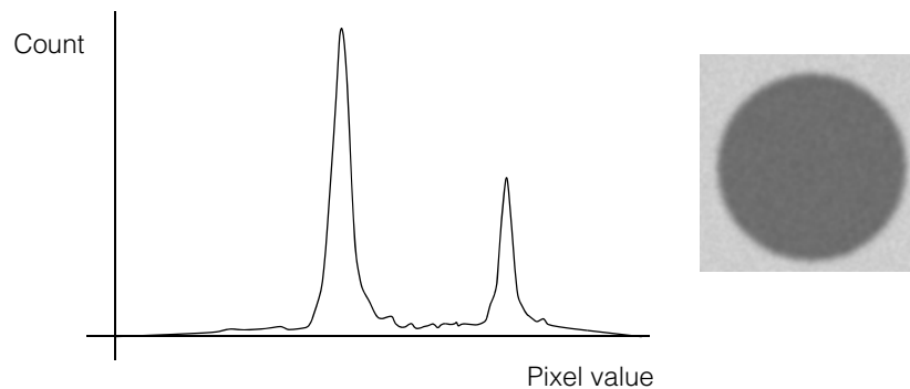
Figure 87. Object image and histogram
