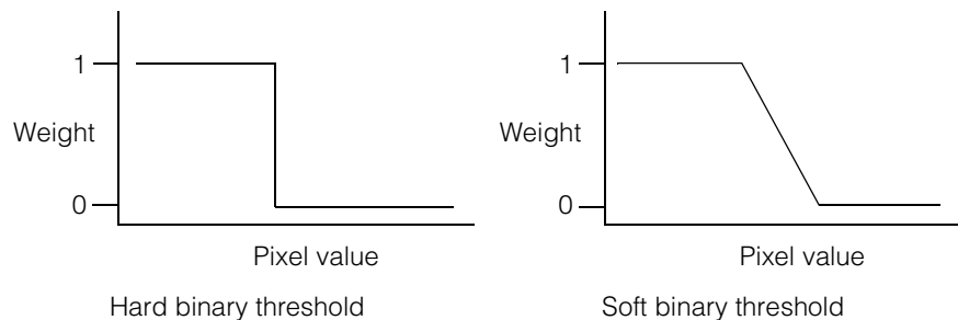
Figure 245. Hard and soft binary thresholds
