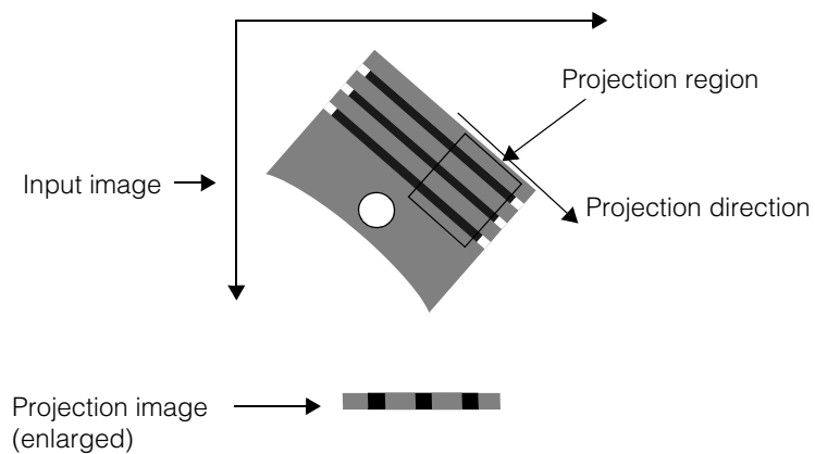
Figure 131. Rotated projection region
