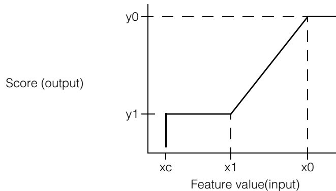
Figure 32. One-sided scoring function
