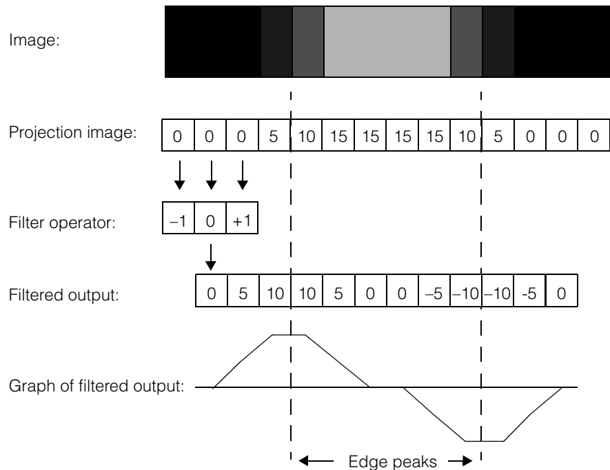
Figure 203. Filtering the projection image
