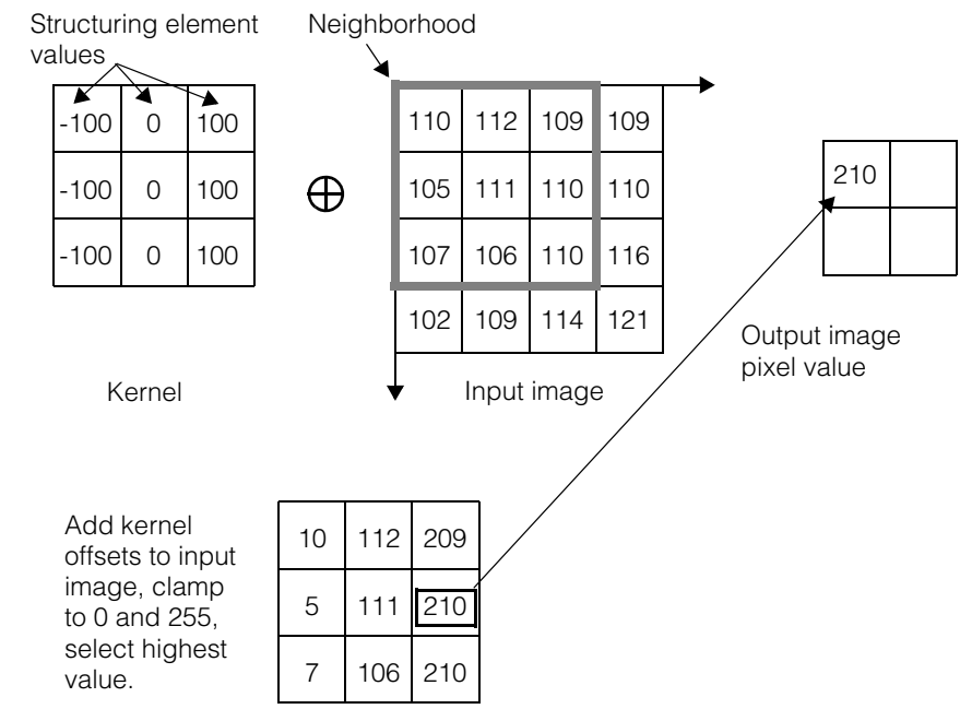
Figure 48. Example of a 3x3 dilation for a single destination pixel
