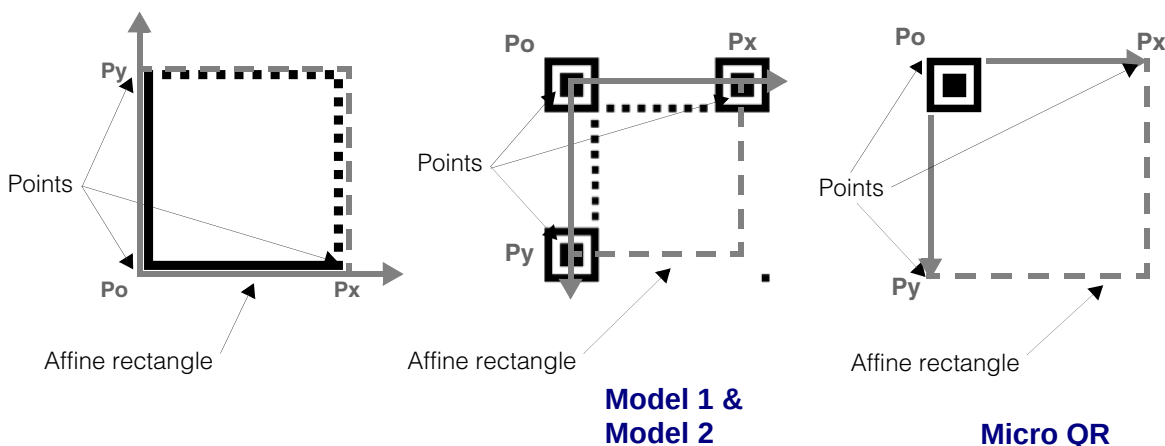
Figure 490. Affine rectangles superimposed on Data Matrix and QR Code finder patterns
