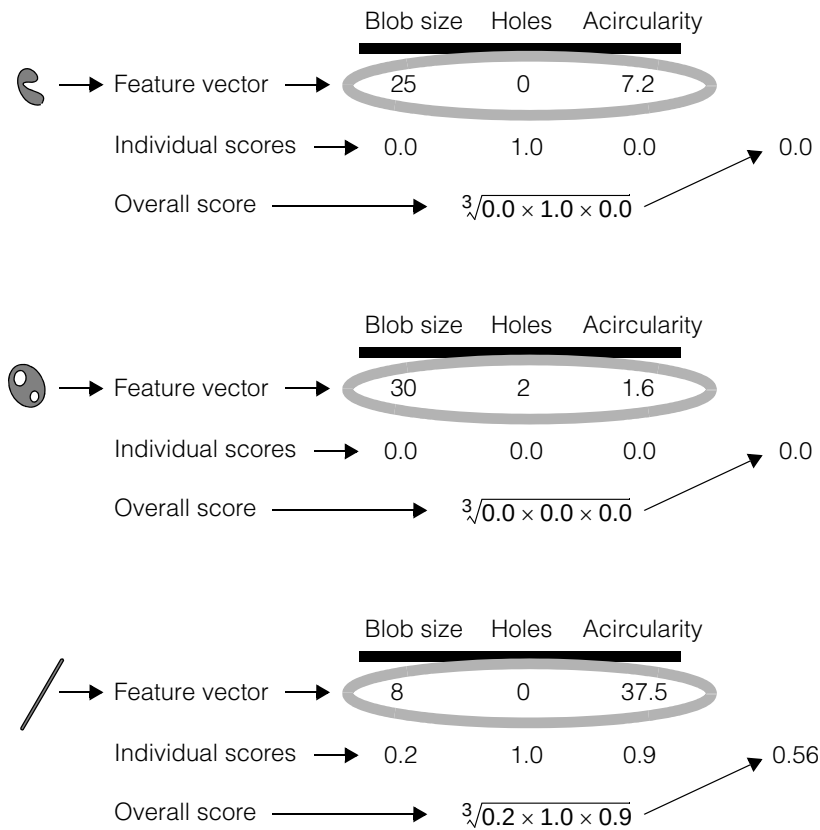
Figure 29. Applying the rule to each feature
