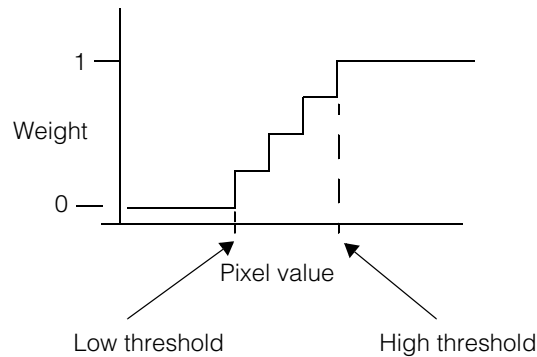
Figure 258. Soft binary thresholding parameters
