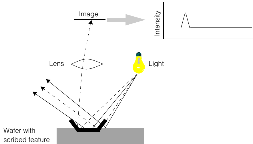
Figure 467. Darkfield lighting
