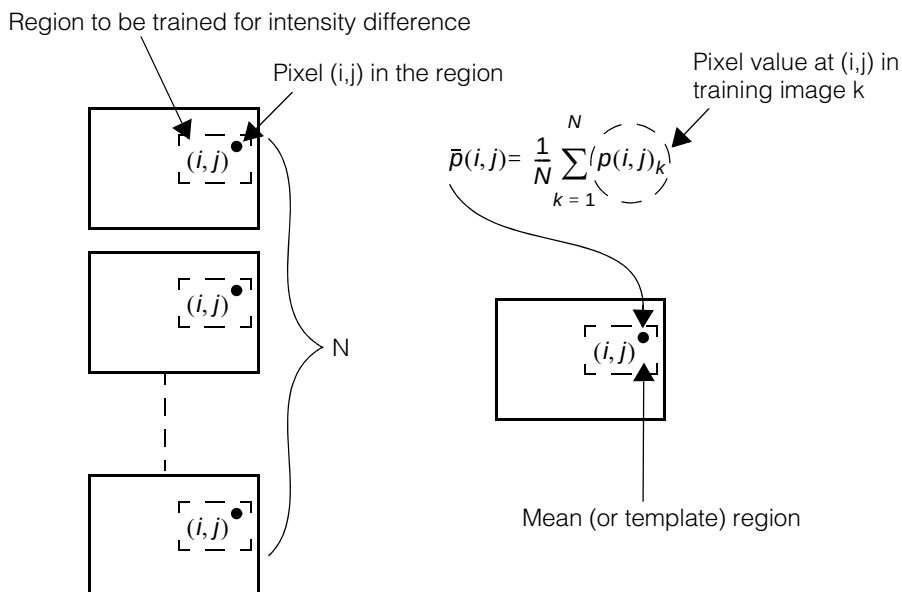
Figure 426. The mean (or template) region for intensity difference training
