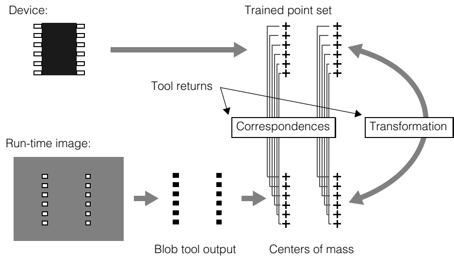
Figure 37. Point Matcher tool application
