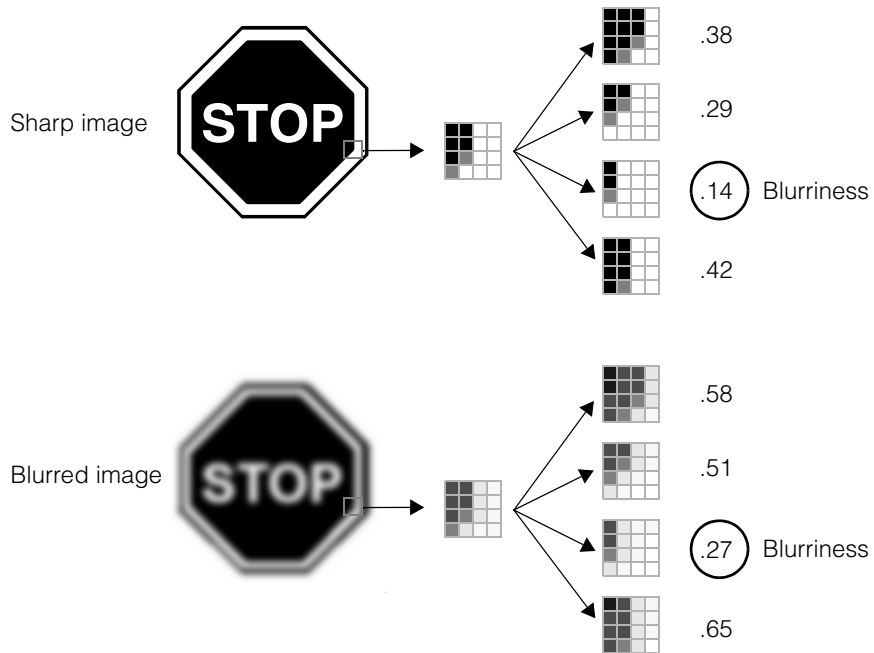
Figure 94. Computing image blurriness in auto-correlation mode
