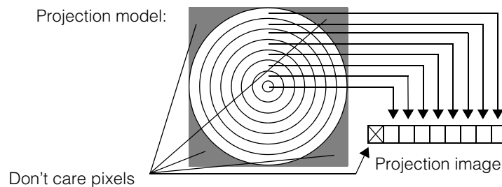
Figure 71. Circular projection model
