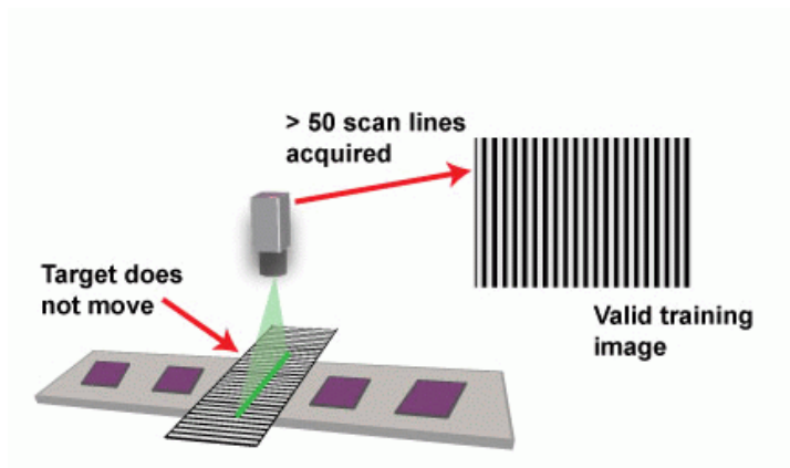
Figure 199. Overview of the training image acquisition process
