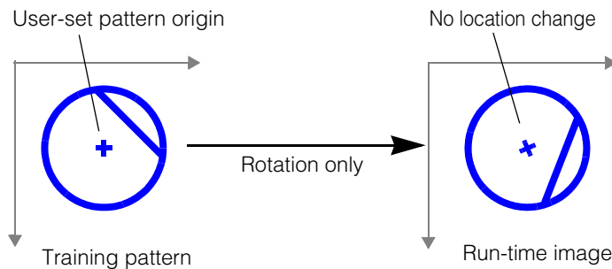
Figure 356. Pattern rotation with origin at pattern center
