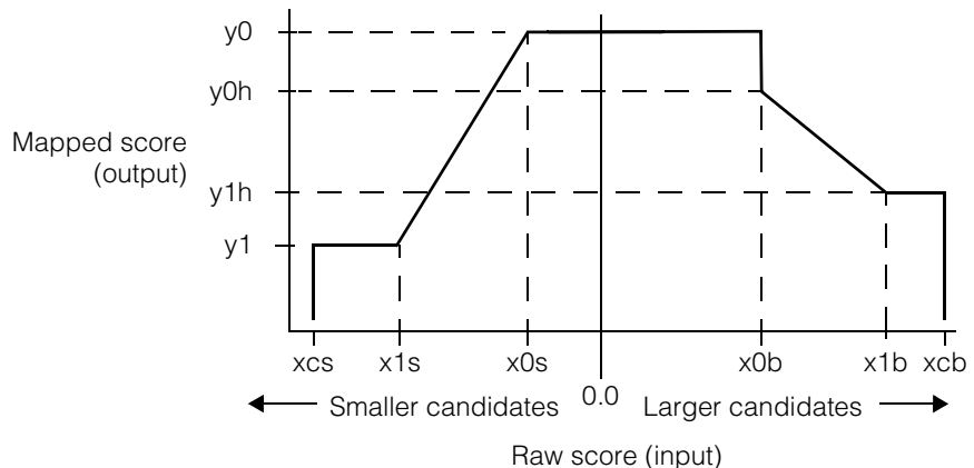
Figure 225. Two-sided scoring function
