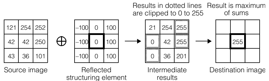
Figure 56. Example of a 3x3 dilation for a single destination pixel
