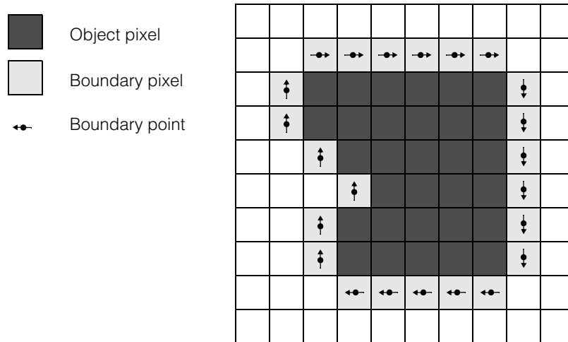
Figure 266. Object, boundary pixels, and boundary points
