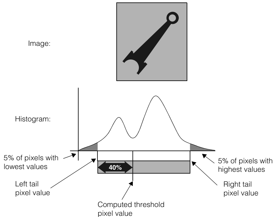
Figure 247. Computing a relative threshold value
