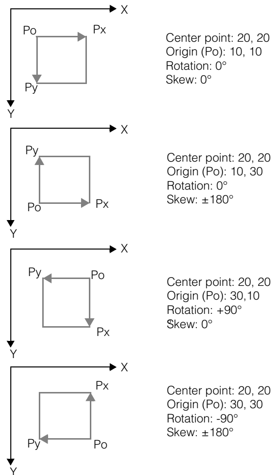
Figure 125. Creating an affine rectangle.
