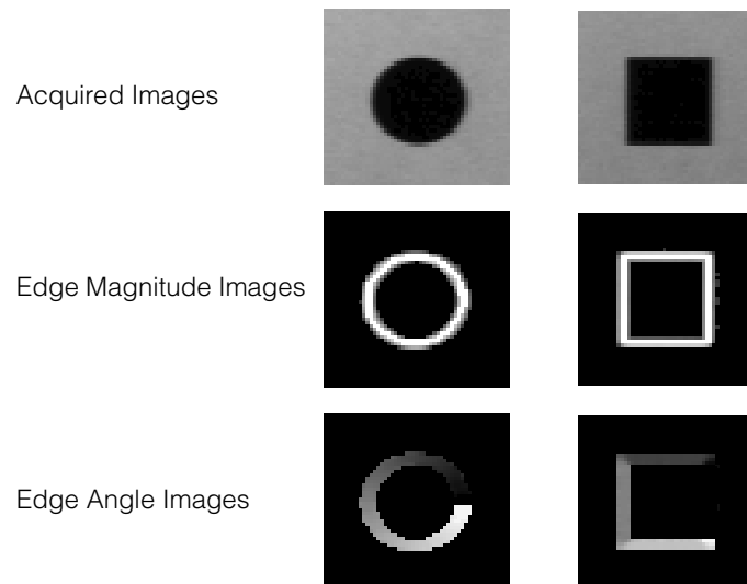
Figure 232. Edge magnitude and angle images
