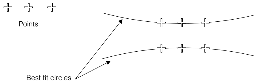
Figure 21. Unstable solution (fitting a circle to three points)
