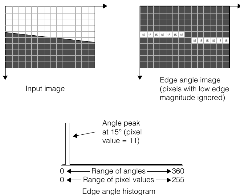
Figure 150. Computing scene angle
