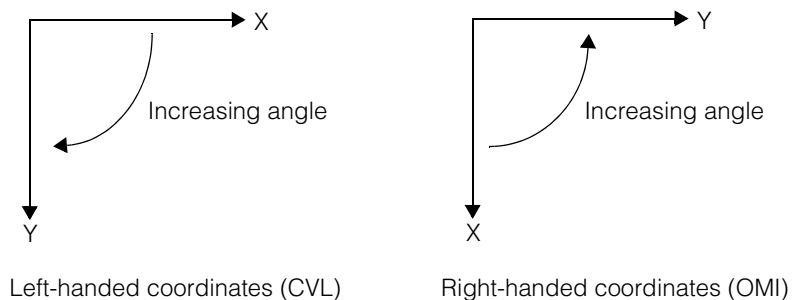
Figure 133. OMI and CVL default coordinate systems
