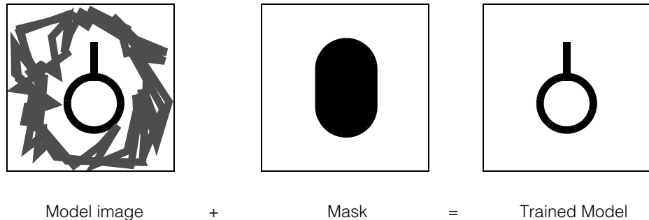
Figure 304. Using a mask image to train a model
