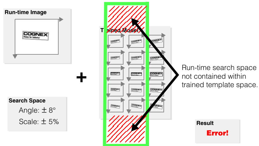
Figure 365. Invalid run-time search space
