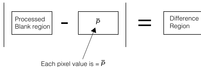
Figure 446. Difference region for blank scene inspection
