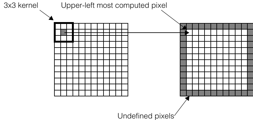
Figure 84. Undefined pixels resulting from ordinary kernel application
