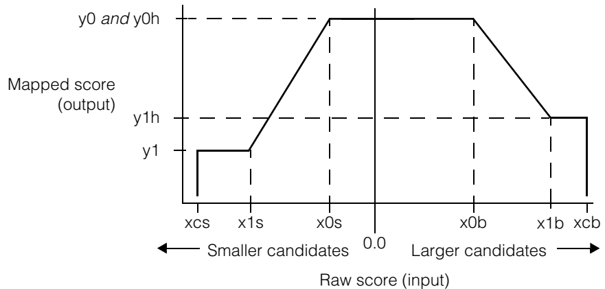
Figure 224. Two-sided scoring function
