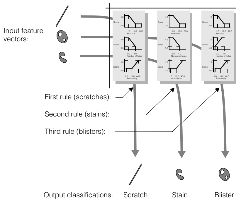
Figure 31. Rules table applied to input feature vectors
