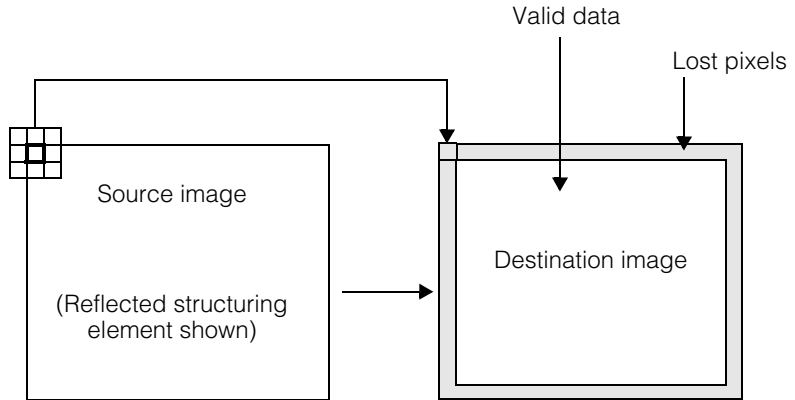
Figure 66. Lost pixels for a single operation with a 3x3 structuring element with origin at center
