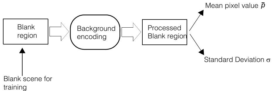
Figure 428. The pre-processing of a training blank scene
