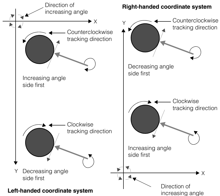
Figure 277. Determining tracking direction from the setting of the decreasingAngleSideFirst parameter
