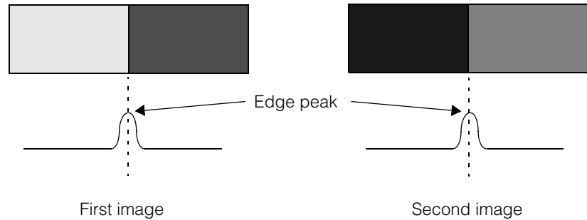
Figure 294. Edge detection with nonlinear brightness change
