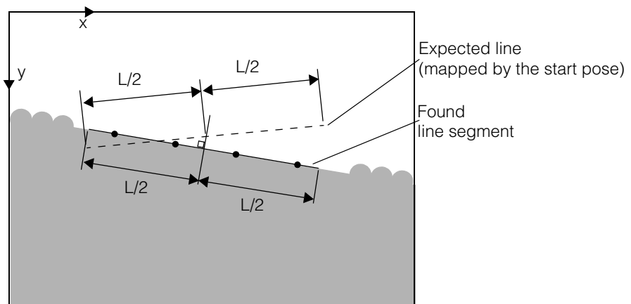
Figure 386. Returned line segment example
