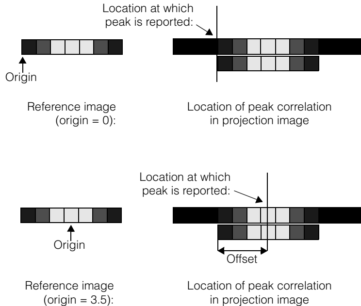
Figure 208. Specifying an origin
