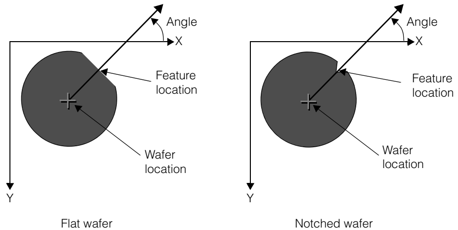
Figure 410. Wafer angle and location and feature location
