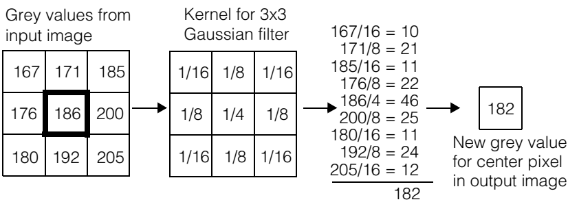
Figure 83. Applying a 3x3 Gaussian kernel
