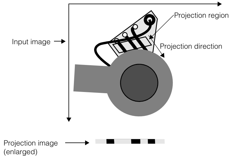
Figure 132. Skewed and rotated projection region
