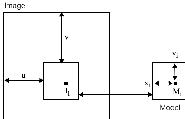
Figure 290. A model and the corresponding portion of the image
