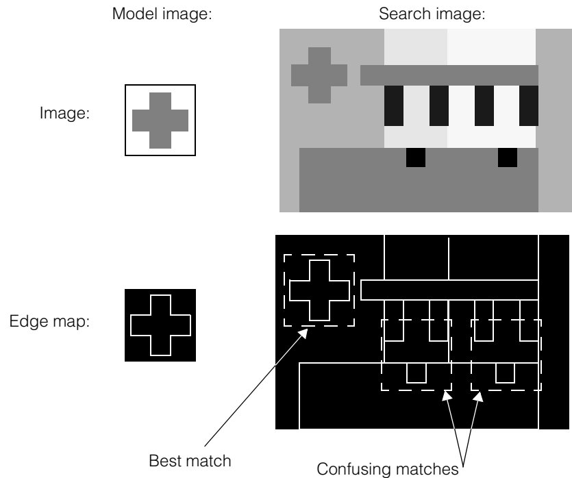
Figure 306. Image confusion in nonlinear mode
