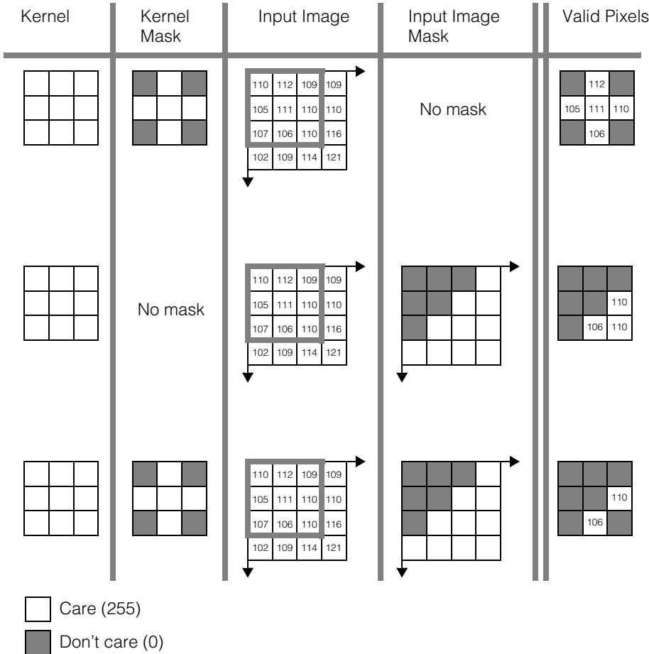
Figure 53. Kernel and input image masks
