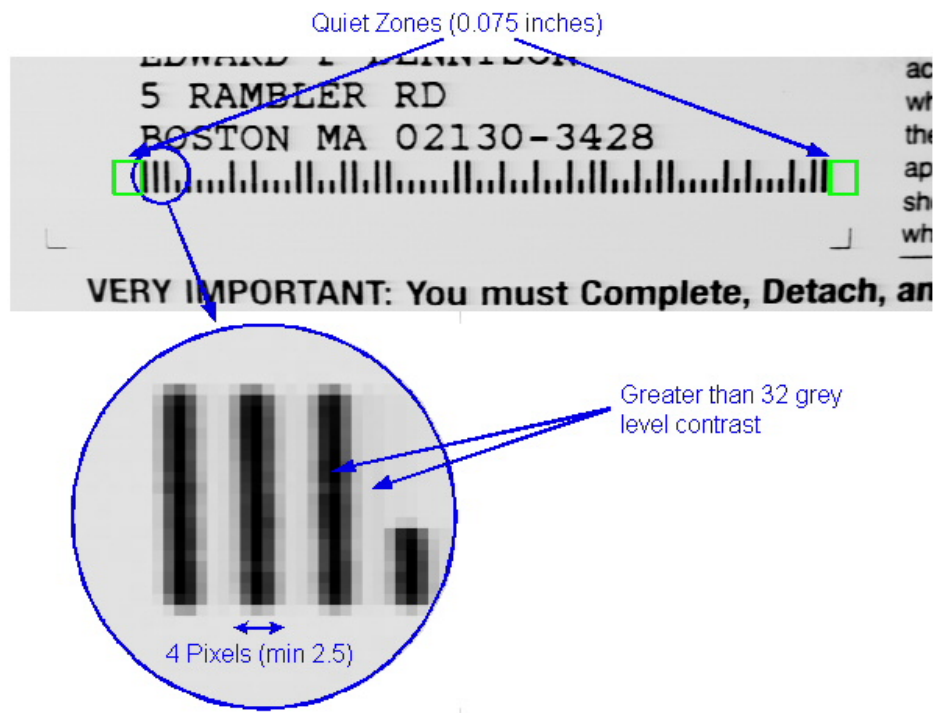
Figure 463. Image requirements (POSTNET)
