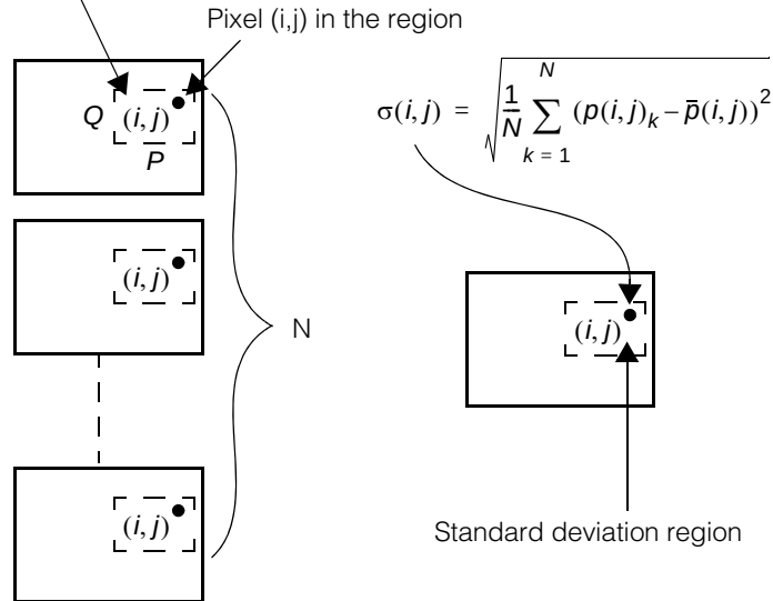
Figure 427. The standard deviation region for intensity difference training
