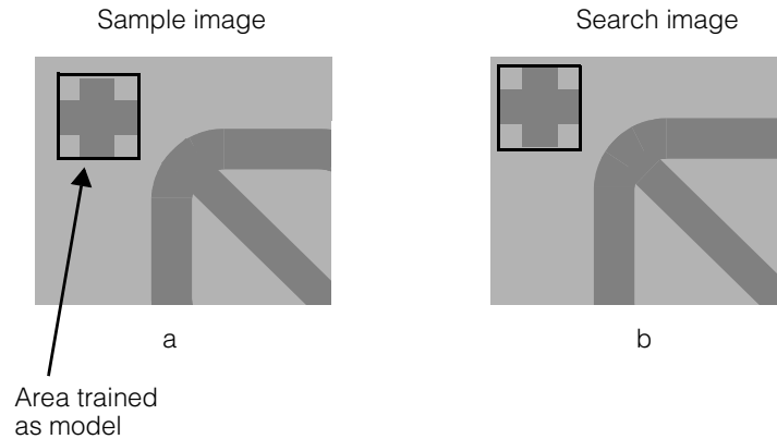
Figure 302. Properly trained model.
