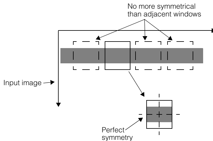
Figure 398. High symmetry with low symmetry score
