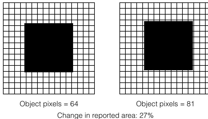
Figure 242. Object position on a pixel grid affects reported area
