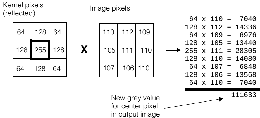
Figure 104. Computing the output pixel value
