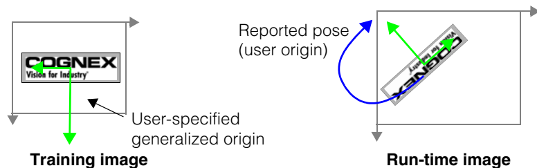
Figure 368. Reported pose for user-specified generalized origin
