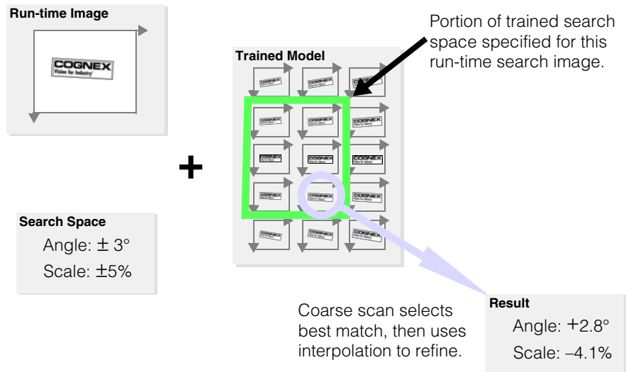
Figure 364. Training-time template generation
