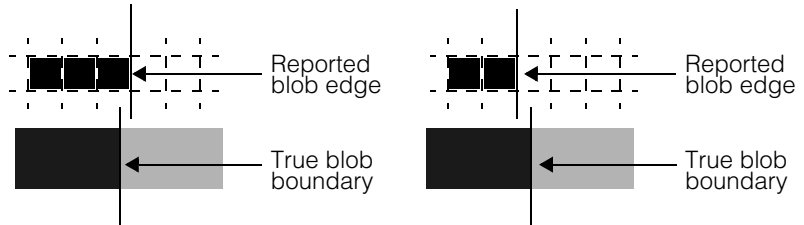
Figure 241. Spatial quantization error
