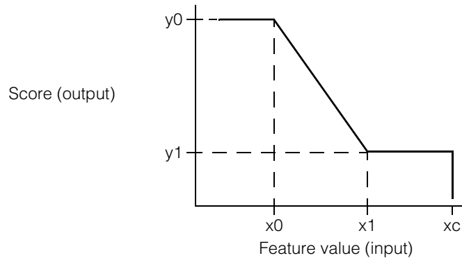
Figure 33. Scoring function with x1 greater than x0
