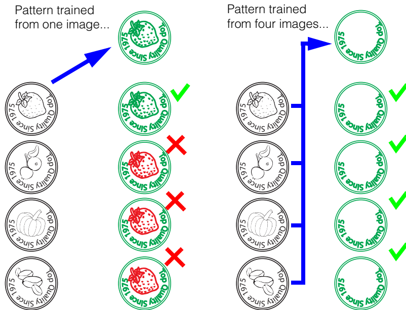
Figure 340. Composite PatMax training for parts with varying features
