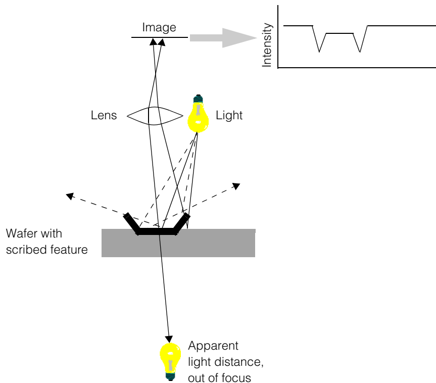
Figure 466. Brightfield lighting
