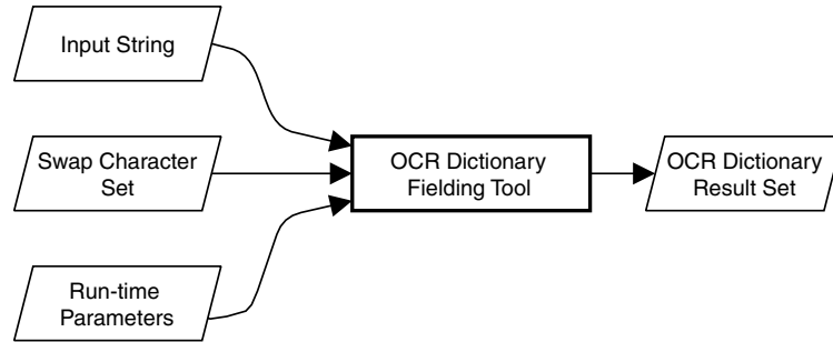
Figure 517. How OCR Dictionary Fielding classes work together
