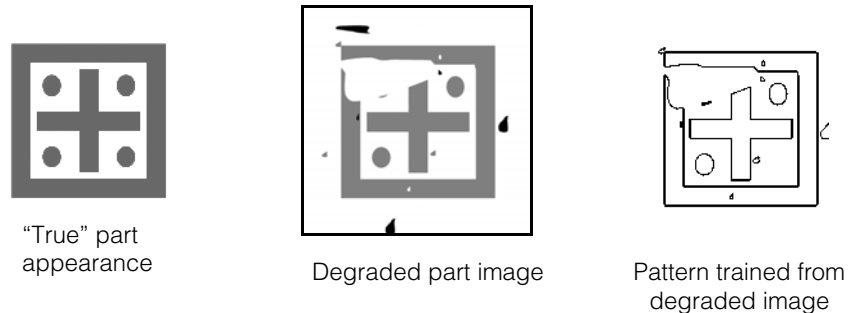
Figure 338. Pattern trained from unrepresentative image
