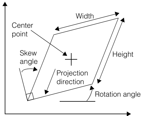
Figure 210. Specifying a projection region
