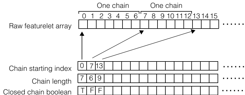
Figure 4. ccFeatureletChainSet internal arrays
