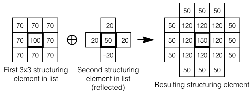
Figure 64. Composing 3x3 structuring elements by dilation
