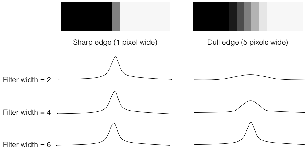
Figure 215. The effect of filter size and edge size on peak size
