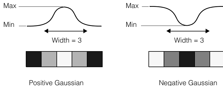
Figure 220. Positive and negative Gaussian reference images
