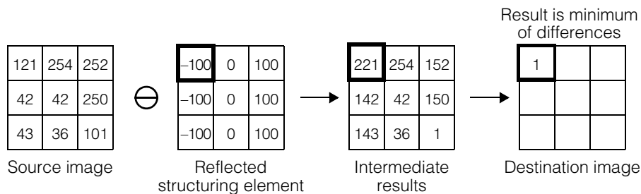
Figure 57. Example of a 3x3 erosion for a single destination pixel
