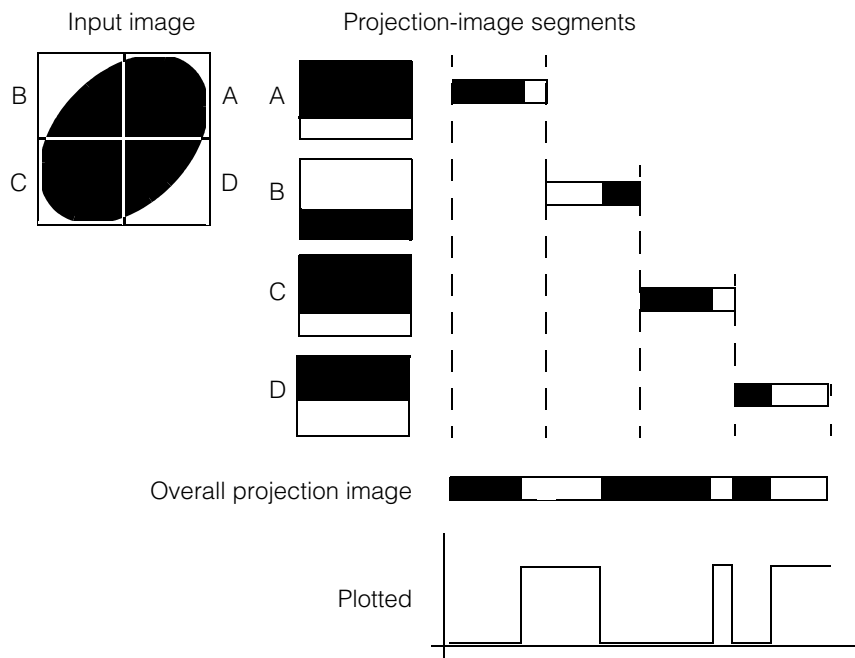
Figure 74. Applying a segmented circular projection model
