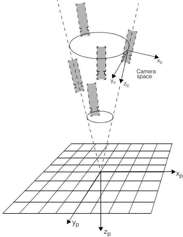
Figure 177. Example camera setup for calibration plate images
