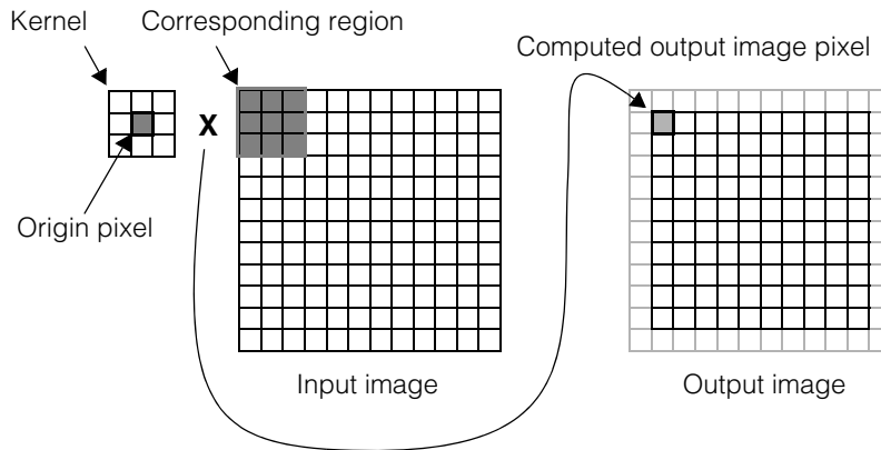
Figure 102. Convolving an image with a kernel
