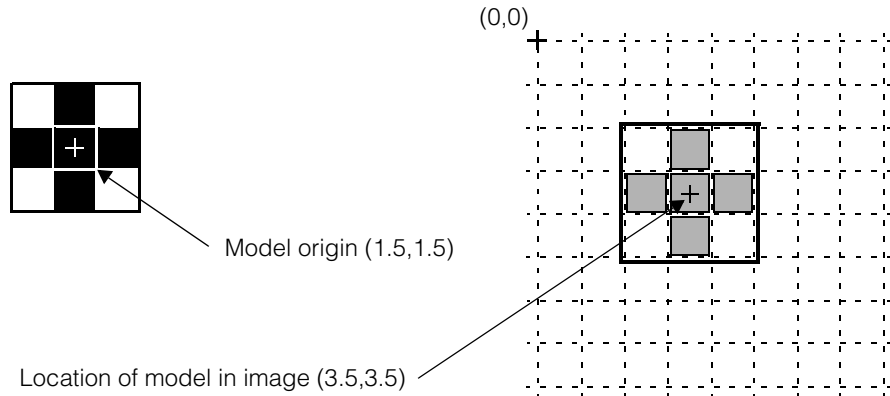
Figure 303. Model origin and model location
