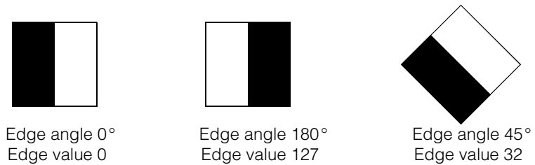
Figure 231. Edge angle and value
