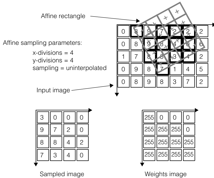
Figure 122. Computing sampled and weights images
