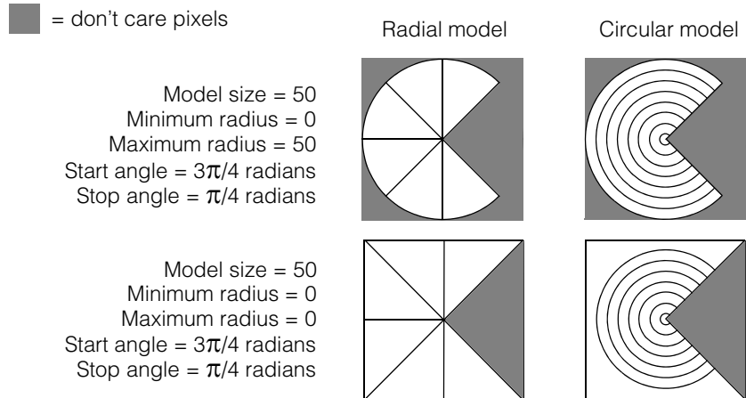
Figure 81. Start and stop angle
