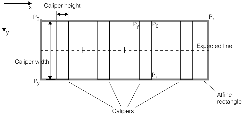
Figure 381. Expected line example using an affine rectangle
