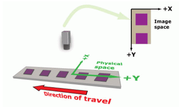
Figure 185. Coordinate spaces associated with line scan camera calibration
