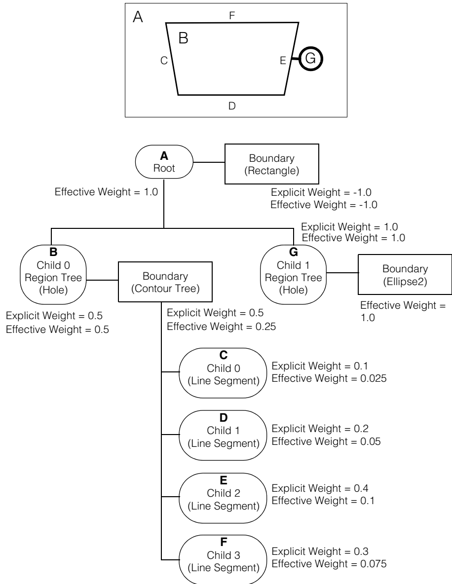
Figure 8. Effective weights of individual nodes in a region tree shape description
