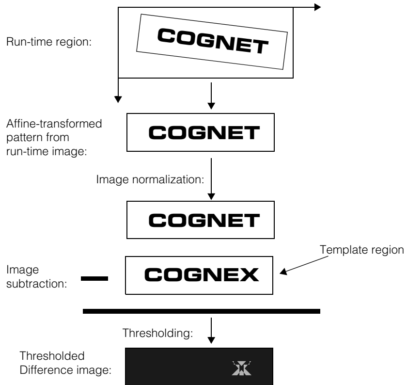
Figure 431. PatInspect intensity difference inspection
