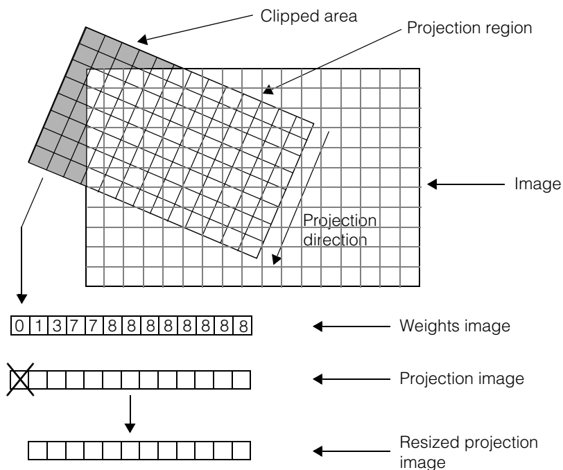
Figure 212. Automatic clipping based on a weights image
