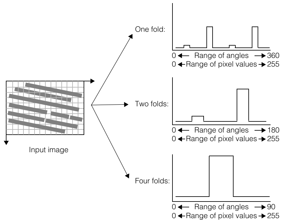
Figure 156. Fold value for rectangular features
