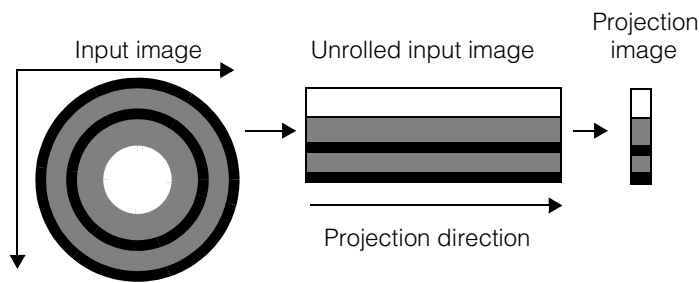
Figure 72. Applying a circular projection model
