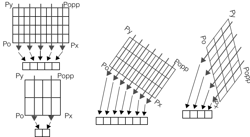
Figure 129. Projection images produced from affine rectangles
