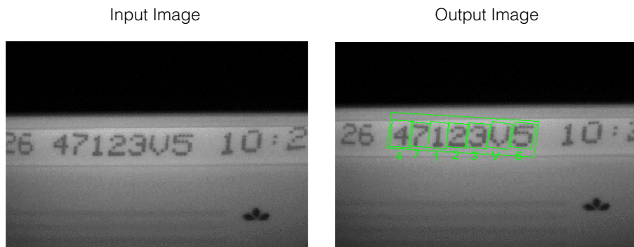
Figure 525. Using the OCVMax tool to verify a string composed of a 5x7 dot-matrix font
