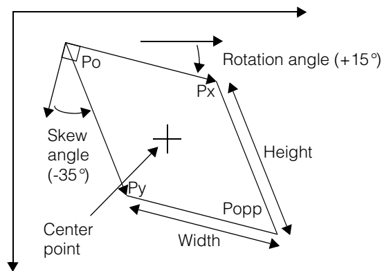
Figure 118. Affine rectangle specified by center point, size, and angles of skew and rotation
