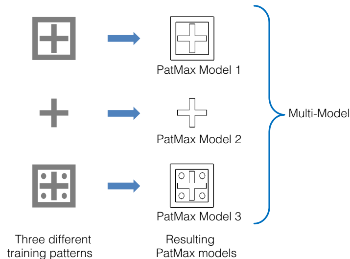
Figure 344. Multi-Model creation in combination with Composite Model training
