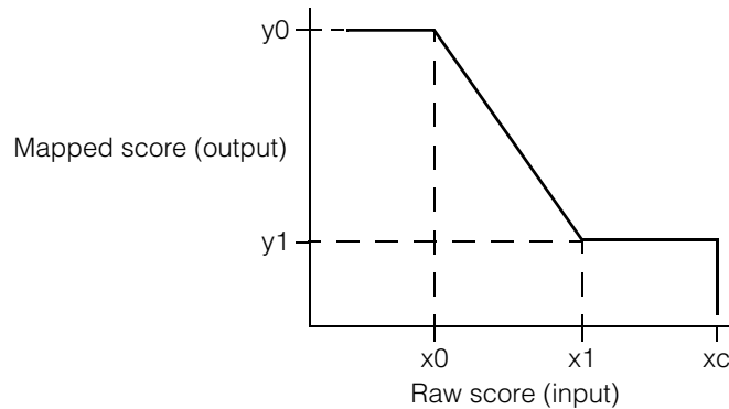
Figure 223. Scoring function with x_1 greater than x_0
