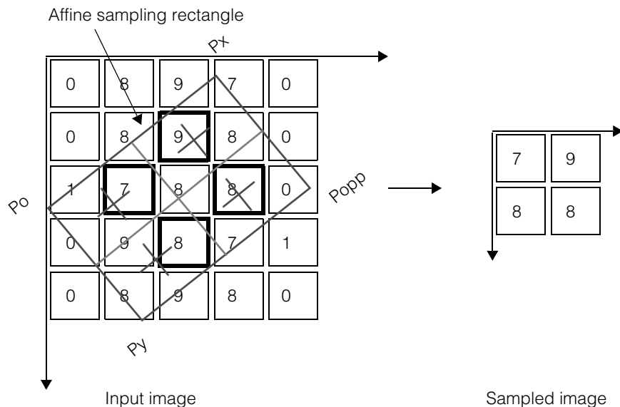
Figure 112. Computing a non-interpolated sample image
